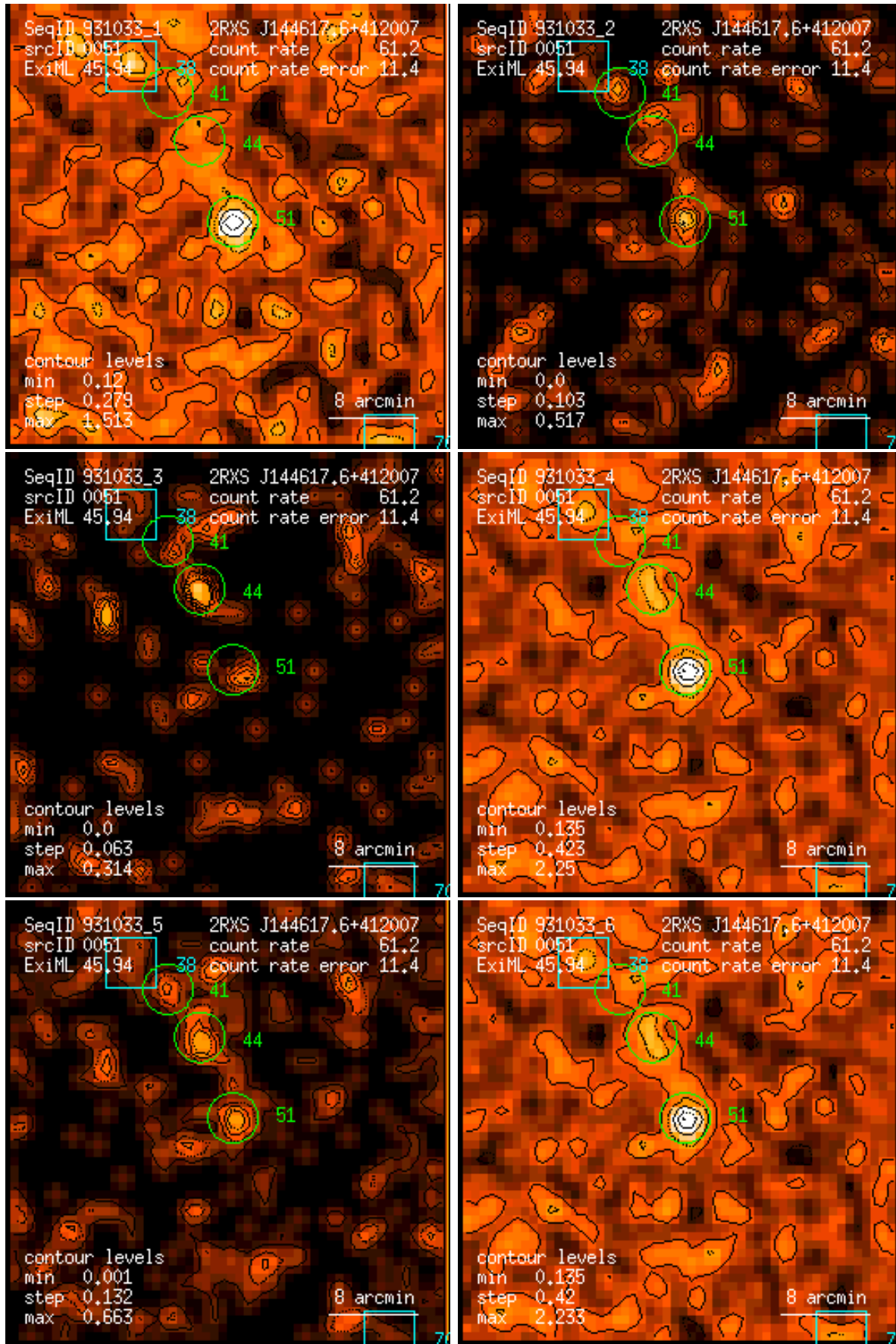
Figure 51: RASS 931033: detection 0051: band rate images, Gaussian filter: (1) PSPC channels 11 – 41, (2) 52 – 90, (3) 91 – 201, (4) 11 – 235, (5) 52 – 201, (6) 11 – 201. Broad band rates in counts/ks. Band rate contour levels in counts/ks/arcmin 2 .
