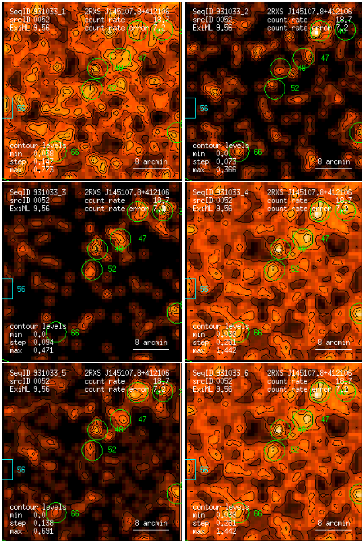
Figure 52: RASS 931033: detection 0052: band rate images, Gaussian filter: (1) PSPC channels 11 – 41, (2) 52 – 90, (3) 91 – 201, (4) 11 – 235, (5) 52 – 201, (6) 11 – 201. Broad band rates in counts/ks. Band rate contour levels in counts/ks/arcmin 2 .
