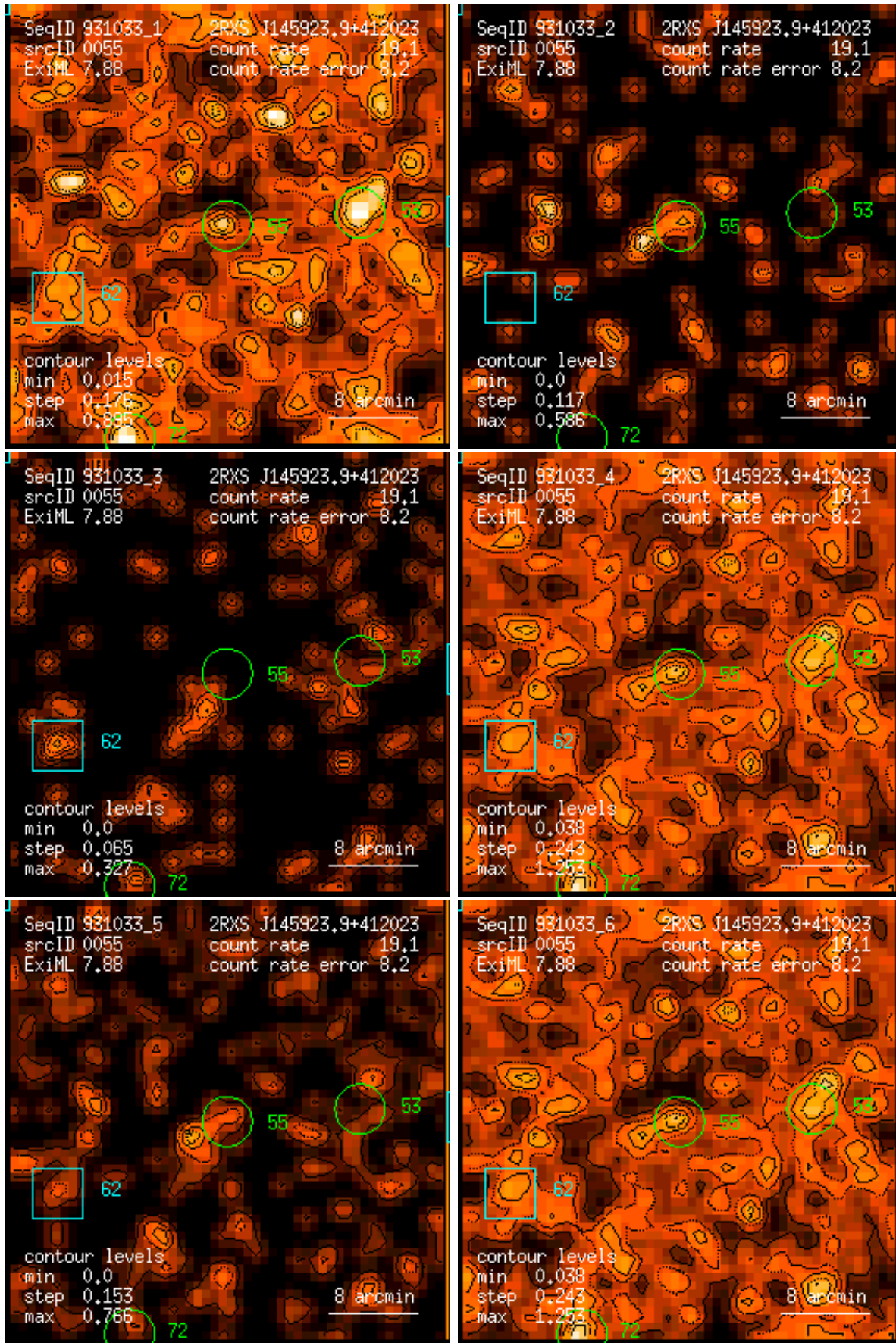
Figure 55: RASS 931033: detection 0055: band rate images, Gaussian filter: (1) PSPC channels 11 – 41, (2) 52 – 90, (3) 91 – 201, (4) 11 – 235, (5) 52 – 201, (6) 11 – 201. Broad band rates in counts/ks. Band rate contour levels in counts/ks/arcmin 2 .
