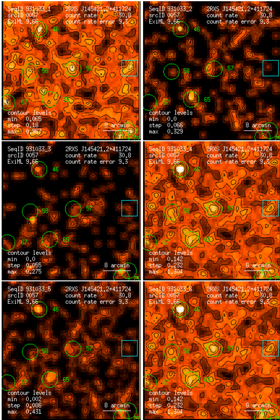
Figure 57: RASS 931033: detection 0057: band rate images, Gaussian filter: (1) PSPC channels 11 – 41, (2) 52 – 90, (3) 91 – 201, (4) 11 – 235, (5) 52 – 201, (6) 11 – 201. Broad band rates in counts/ks. Band rate contour levels in counts/ks/arcmin 2 .
