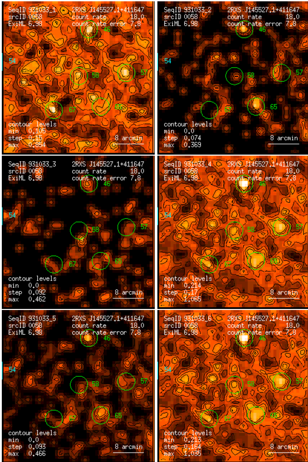
Figure 58: RASS 931033: detection 0058: band rate images, Gaussian filter: (1) PSPC channels 11 – 41, (2) 52 – 90, (3) 91 – 201, (4) 11 – 235, (5) 52 – 201, (6) 11 – 201. Broad band rates in counts/ks. Band rate contour levels in counts/ks/arcmin 2 .
