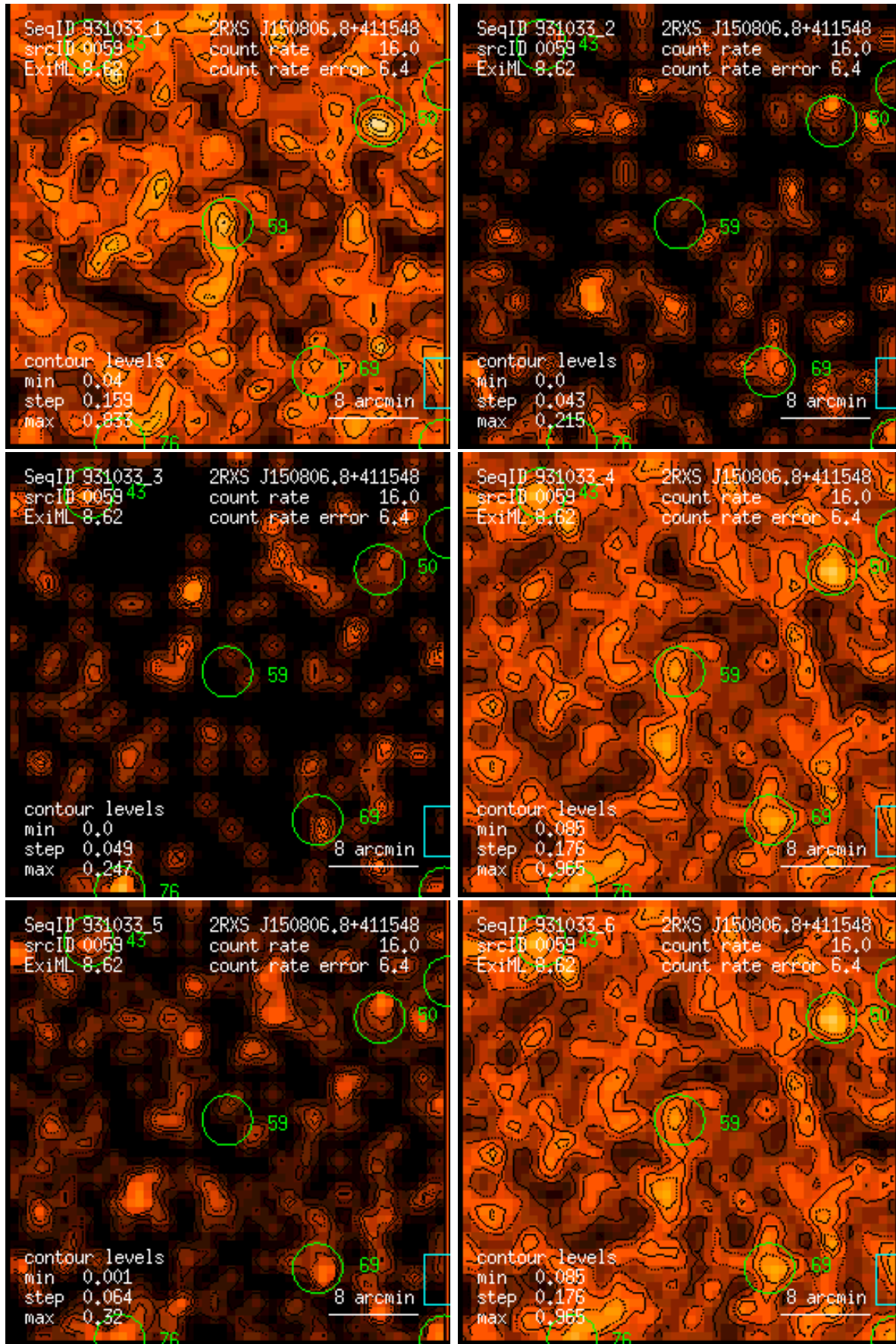
Figure 59: RASS 931033: detection 0059: band rate images, Gaussian filter: (1) PSPC channels 11 – 41, (2) 52 – 90, (3) 91 – 201, (4) 11 – 235, (5) 52 – 201, (6) 11 – 201. Broad band rates in counts/ks. Band rate contour levels in counts/ks/arcmin 2 .
