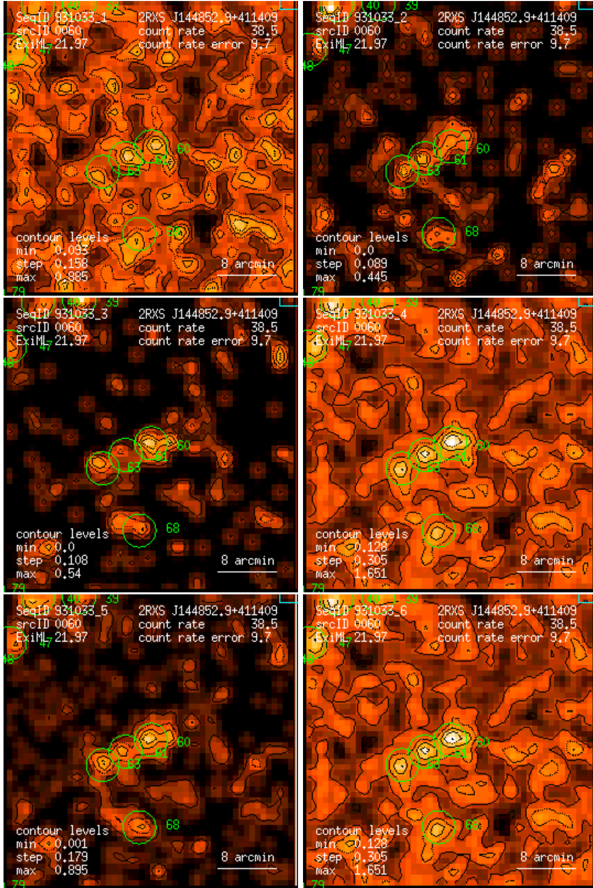
Figure 60: RASS 931033: detection 0060: band rate images, Gaussian filter: (1) PSPC channels 11 – 41, (2) 52 – 90, (3) 91 – 201, (4) 11 – 235, (5) 52 – 201, (6) 11 – 201. Broad band rates in counts/ks. Band rate contour levels in counts/ks/arcmin 2 .
