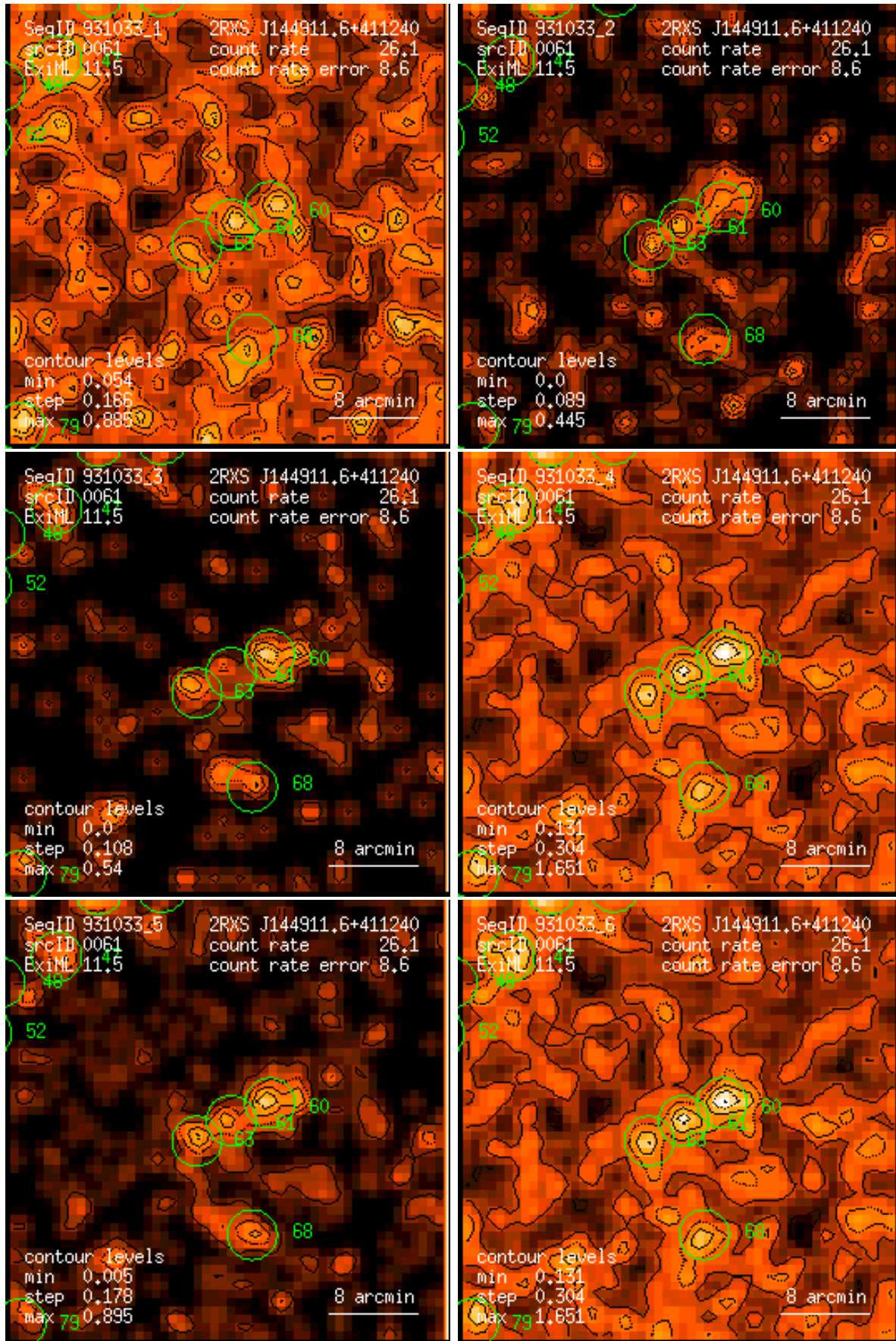
Figure 61: RASS 931033: detection 0061: band rate images, Gaussian filter: (1) PSPC channels 11 – 41, (2) 52 – 90, (3) 91 – 201, (4) 11 – 235, (5) 52 – 201, (6) 11 – 201. Broad band rates in counts/ks. Band rate contour levels in counts/ks/arcmin 2 .
