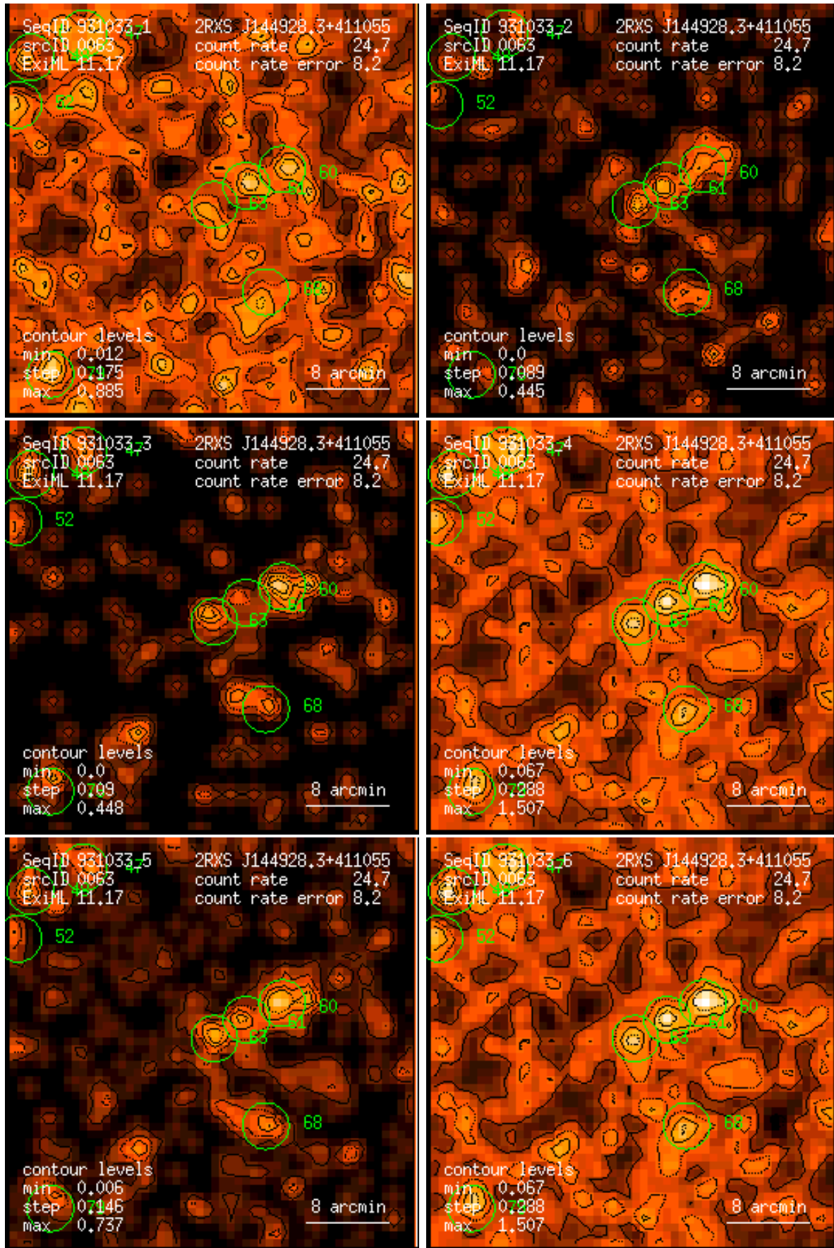
Figure 63: RASS 931033: detection 0063: band rate images, Gaussian filter: (1) PSPC channels 11 – 41, (2) 52 – 90, (3) 91 – 201, (4) 11 – 235, (5) 52 – 201, (6) 11 – 201. Broad band rates in counts/ks. Band rate contour levels in counts/ks/arcmin 2 .
