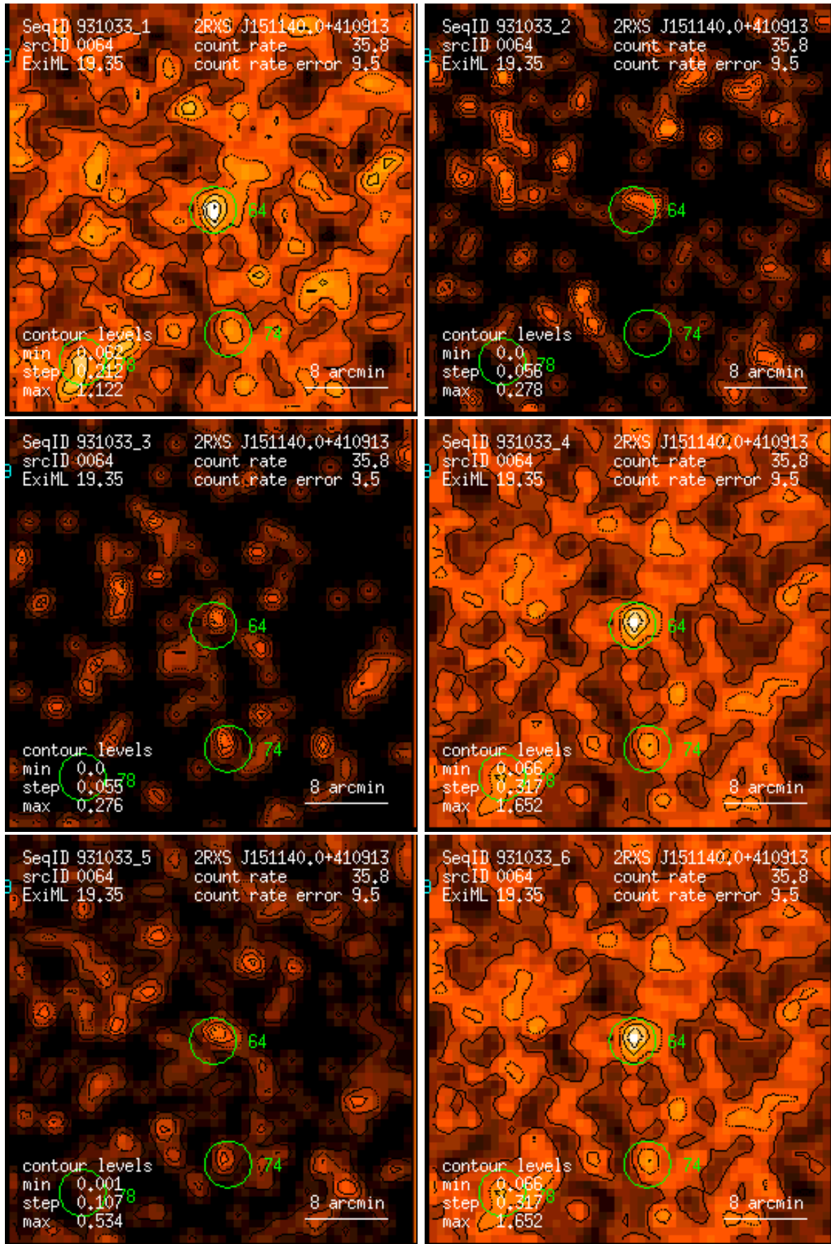
Figure 64: RASS 931033: detection 0064: band rate images, Gaussian filter: (1) PSPC channels 11 – 41, (2) 52 – 90, (3) 91 – 201, (4) 11 – 235, (5) 52 – 201, (6) 11 – 201. Broad band rates in counts/ks. Band rate contour levels in counts/ks/arcmin 2 .
