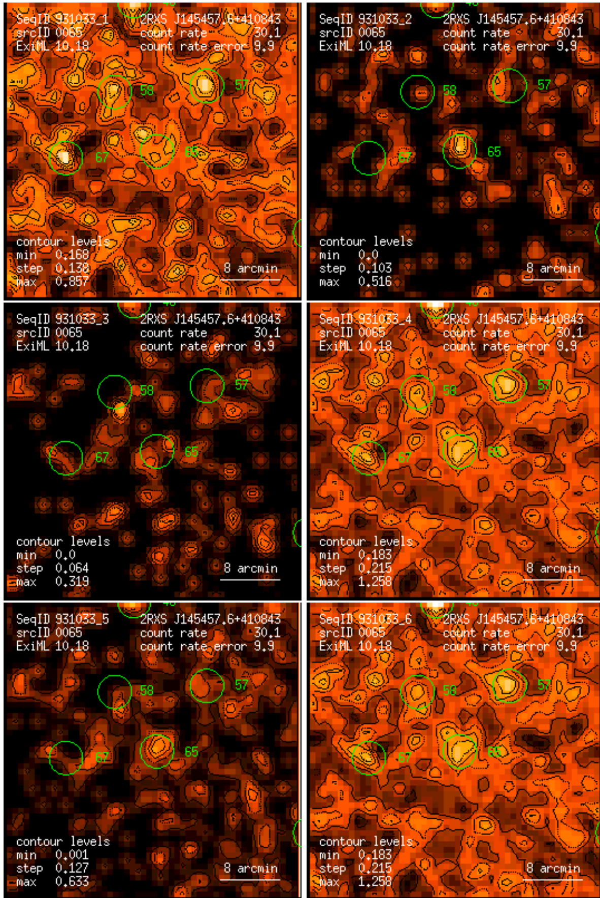
Figure 65: RASS 931033: detection 0065: band rate images, Gaussian filter: (1) PSPC channels 11 – 41, (2) 52 – 90, (3) 91 – 201, (4) 11 – 235, (5) 52 – 201, (6) 11 – 201. Broad band rates in counts/ks. Band rate contour levels in counts/ks/arcmin 2 .
