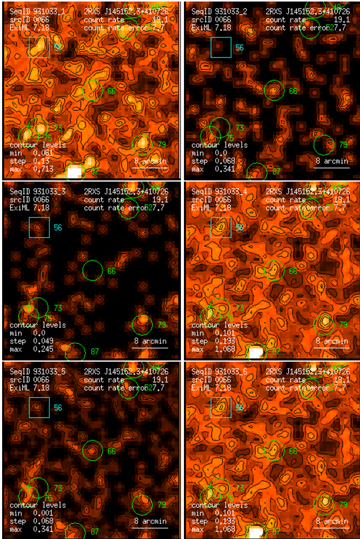
Figure 66: RASS 931033: detection 0066: band rate images, Gaussian filter: (1) PSPC channels 11 – 41, (2) 52 – 90, (3) 91 – 201, (4) 11 – 235, (5) 52 – 201, (6) 11 – 201. Broad band rates in counts/ks. Band rate contour levels in counts/ks/arcmin 2 .
