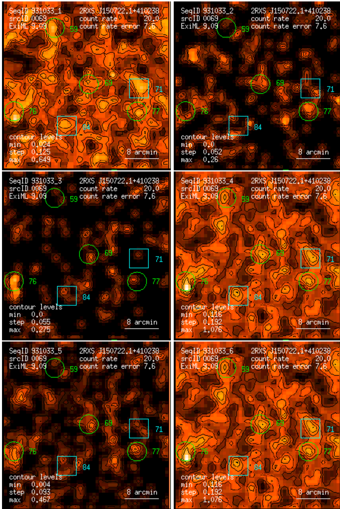
Figure 69: RASS 931033: detection 0069: band rate images, Gaussian filter: (1) PSPC channels 11 – 41, (2) 52 – 90, (3) 91 – 201, (4) 11 – 235, (5) 52 – 201, (6) 11 – 201. Broad band rates in counts/ks. Band rate contour levels in counts/ks/arcmin 2 .
