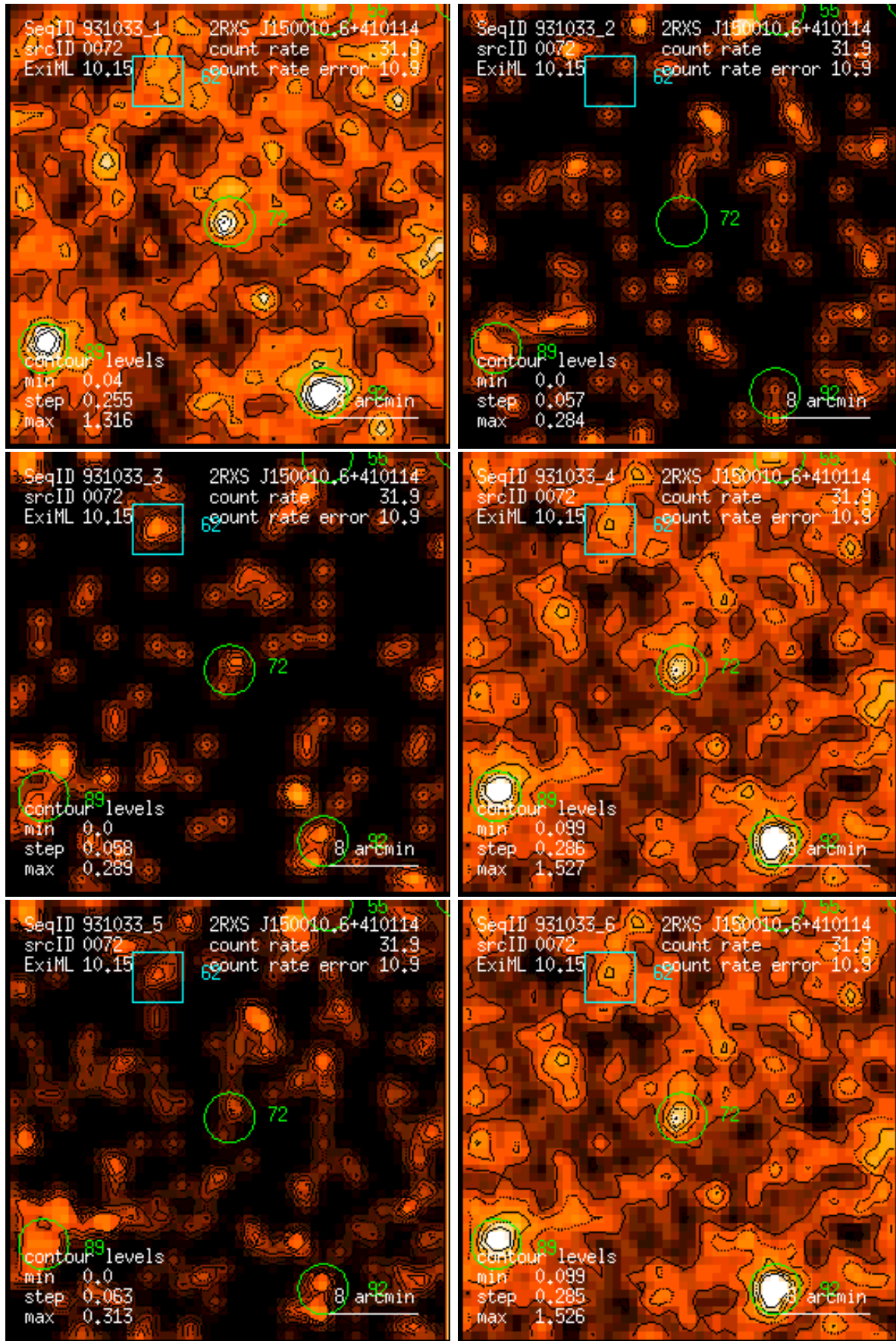
Figure 72: RASS 931033: detection 0072: band rate images, Gaussian filter: (1) PSPC channels 11 – 41, (2) 52 – 90, (3) 91 – 201, (4) 11 – 235, (5) 52 – 201, (6) 11 – 201. Broad band rates in counts/ks. Band rate contour levels in counts/ks/arcmin 2 .
