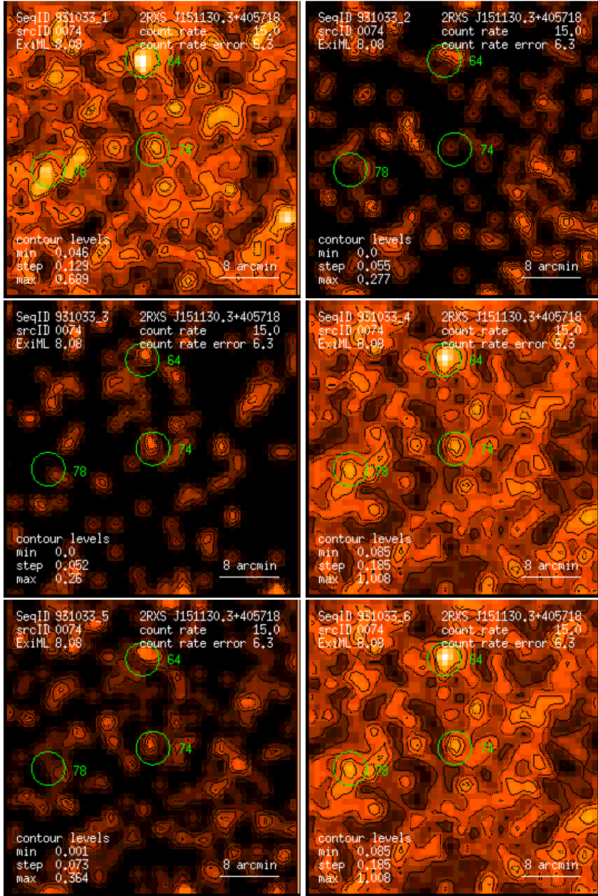
Figure 74: RASS 931033: detection 0074: band rate images, Gaussian filter: (1) PSPC channels 11 – 41, (2) 52 – 90, (3) 91 – 201, (4) 11 – 235, (5) 52 – 201, (6) 11 – 201. Broad band rates in counts/ks. Band rate contour levels in counts/ks/arcmin 2 .
