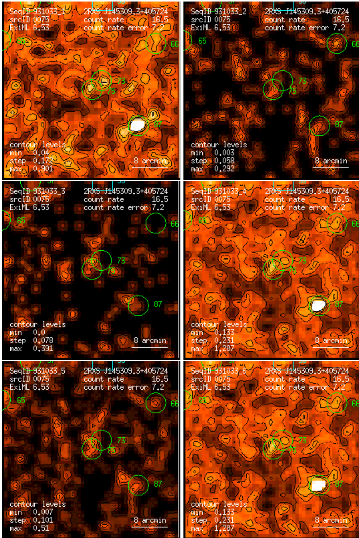
Figure 75: RASS 931033: detection 0075: band rate images, Gaussian filter: (1) PSPC channels 11 – 41, (2) 52 – 90, (3) 91 – 201, (4) 11 – 235, (5) 52 – 201, (6) 11 – 201. Broad band rates in counts/ks. Band rate contour levels in counts/ks/arcmin 2 .
