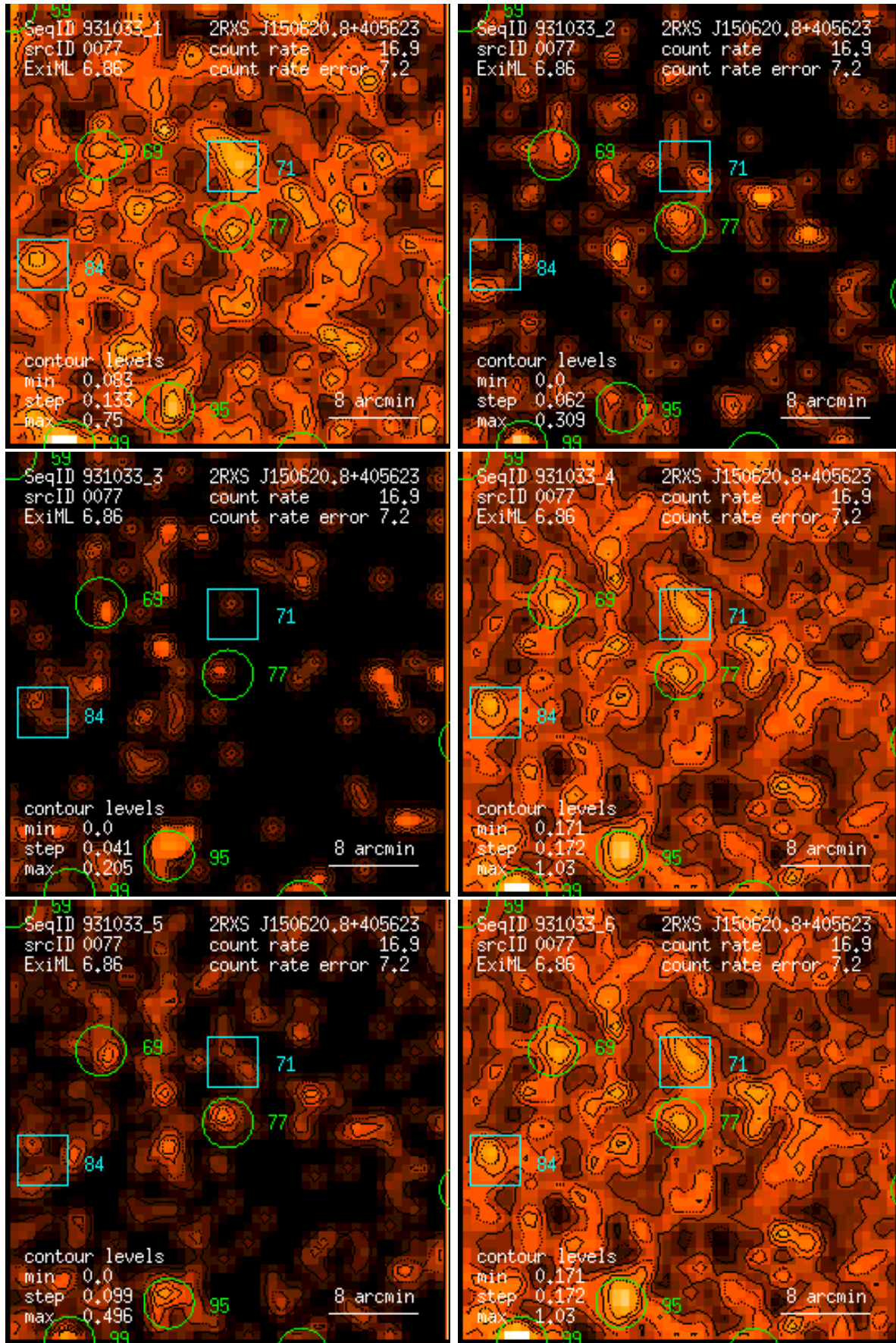
Figure 77: RASS 931033: detection 0077: band rate images, Gaussian filter: (1) PSPC channels 11 – 41, (2) 52 – 90, (3) 91 – 201, (4) 11 – 235, (5) 52 – 201, (6) 11 – 201. Broad band rates in counts/ks. Band rate contour levels in counts/ks/arcmin 2 .
