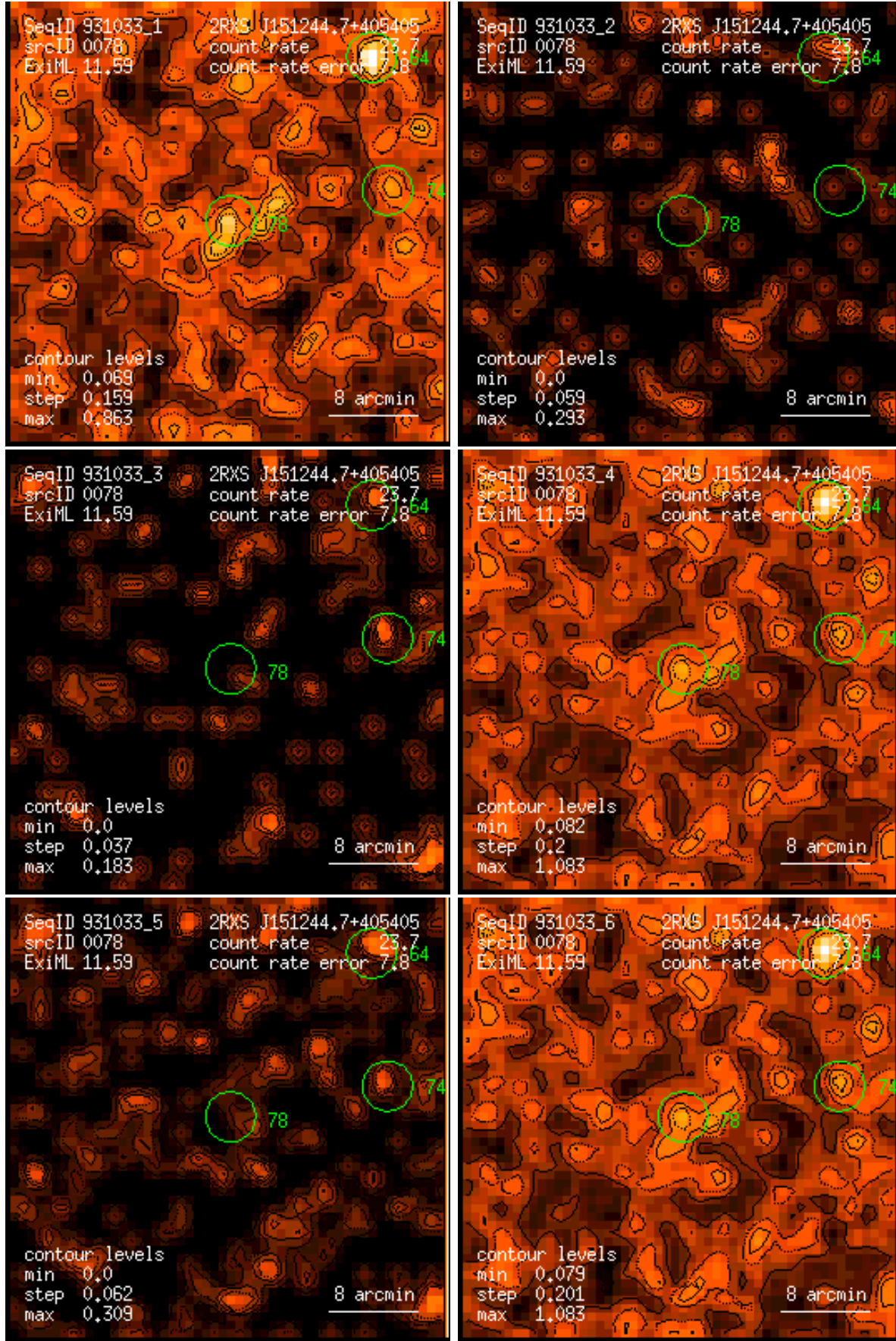
Figure 78: RASS 931033: detection 0078: band rate images, Gaussian filter: (1) PSPC channels 11 – 41, (2) 52 – 90, (3) 91 – 201, (4) 11 – 235, (5) 52 – 201, (6) 11 – 201. Broad band rates in counts/ks. Band rate contour levels in counts/ks/arcmin 2 .
