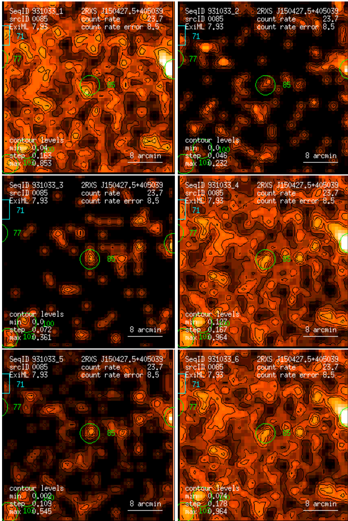
Figure 85: RASS 931033: detection 0085: band rate images, Gaussian filter: (1) PSPC channels 11 – 41, (2) 52 – 90, (3) 91 – 201, (4) 11 – 235, (5) 52 – 201, (6) 11 – 201. Broad band rates in counts/ks. Band rate contour levels in counts/ks/arcmin 2 .
