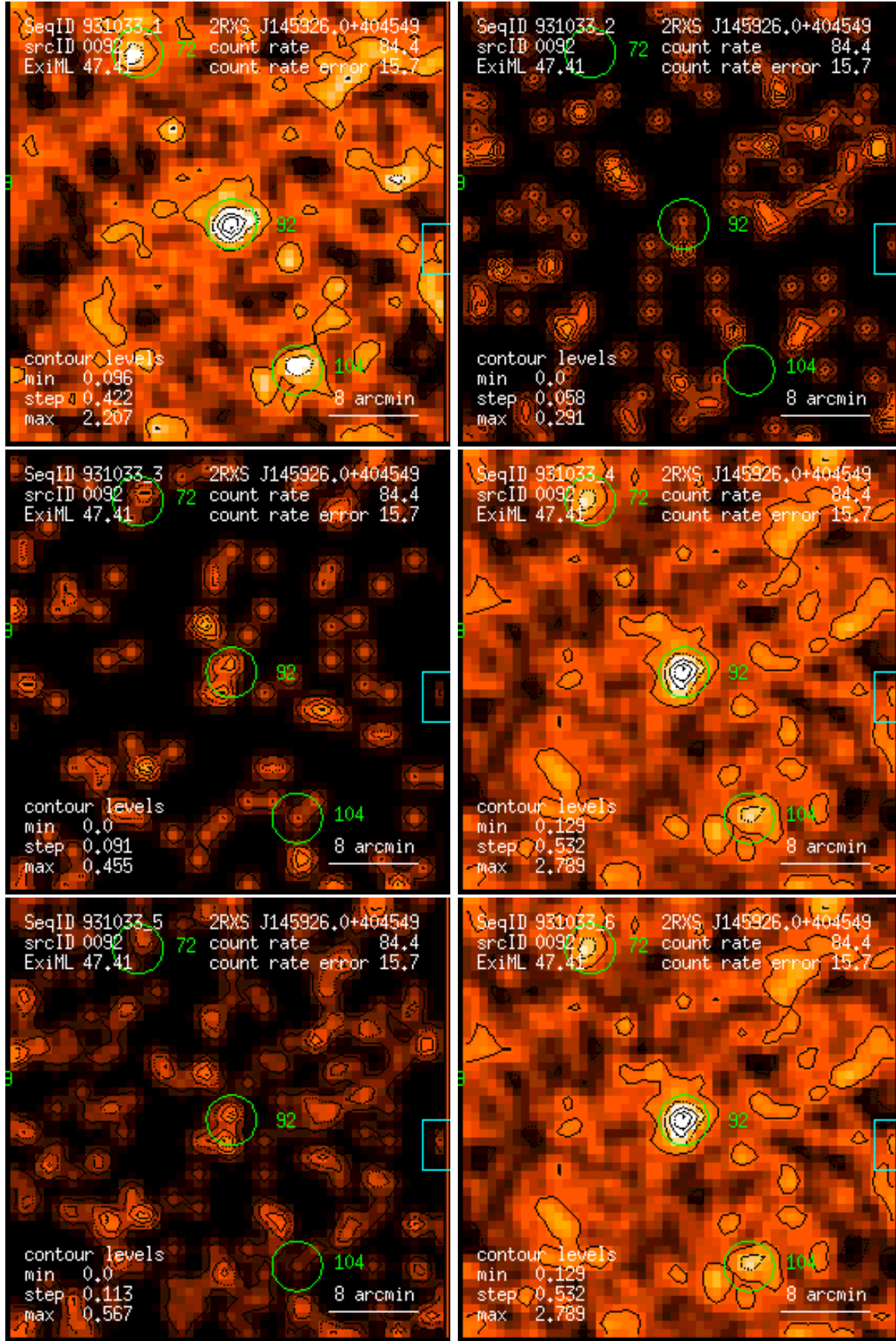
Figure 92: RASS 931033: detection 0092: band rate images, Gaussian filter: (1) PSPC channels 11 – 41, (2) 52 – 90, (3) 91 – 201, (4) 11 – 235, (5) 52 – 201, (6) 11 – 201. Broad band rates in counts/ks. Band rate contour levels in counts/ks/arcmin 2 .
