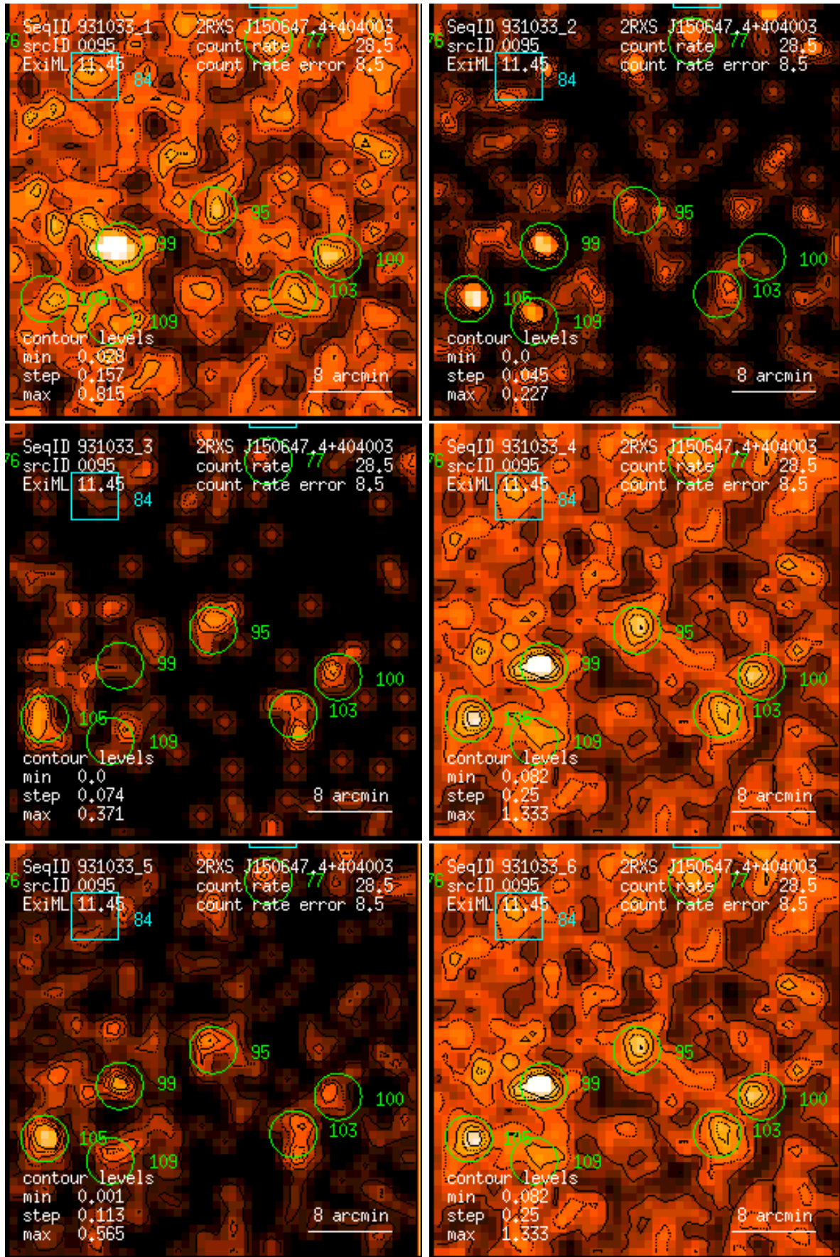
Figure 95: RASS 931033: detection 0095: band rate images, Gaussian filter: (1) PSPC channels 11 – 41, (2) 52 – 90, (3) 91 – 201, (4) 11 – 235, (5) 52 – 201, (6) 11 – 201. Broad band rates in counts/ks. Band rate contour levels in counts/ks/arcmin 2 .
