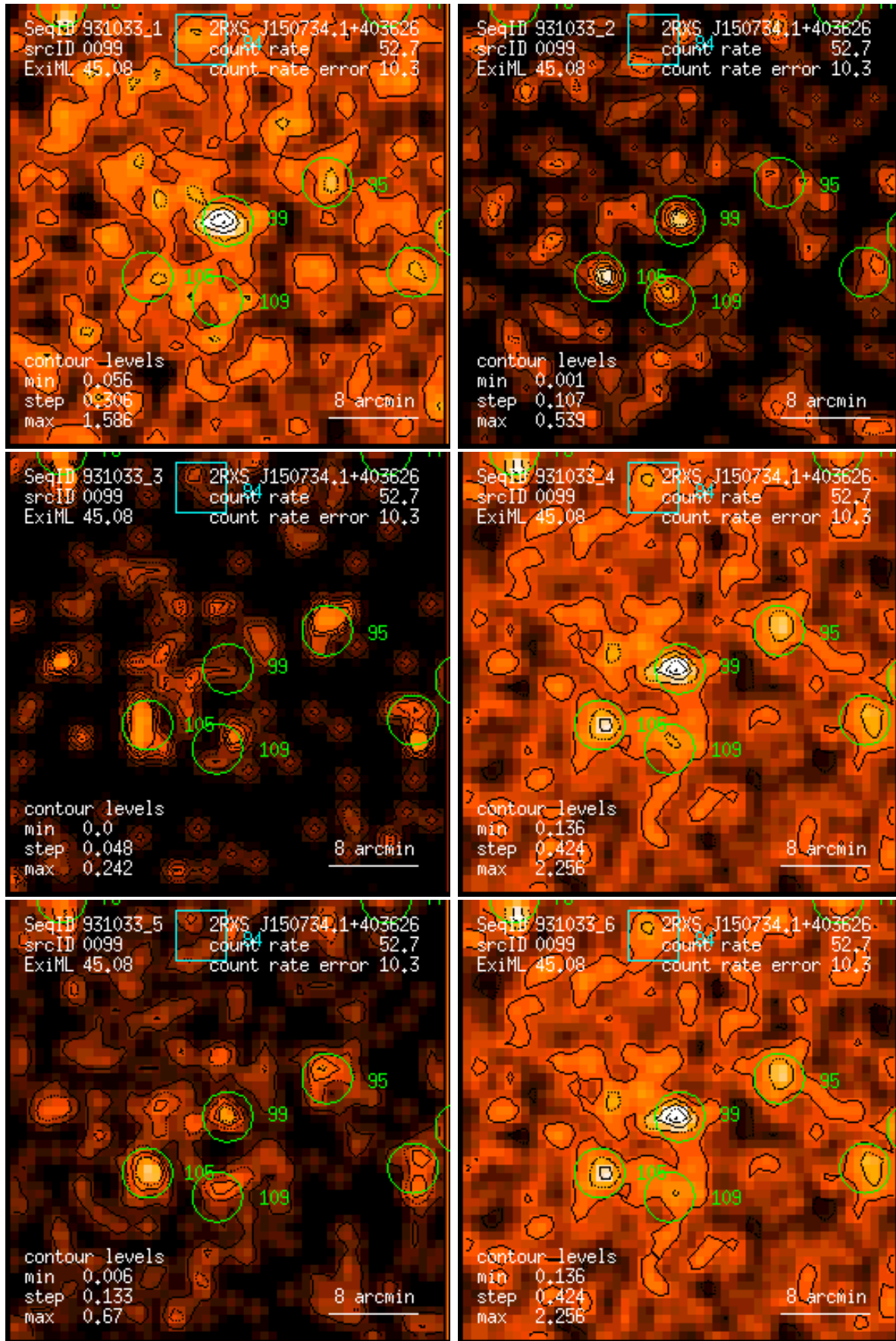
Figure 99: RASS 931033: detection 0099: band rate images, Gaussian filter: (1) PSPC channels 11 – 41, (2) 52 – 90, (3) 91 – 201, (4) 11 – 235, (5) 52 – 201, (6) 11 – 201. Broad band rates in counts/ks. Band rate contour levels in counts/ks/arcmin 2 .
