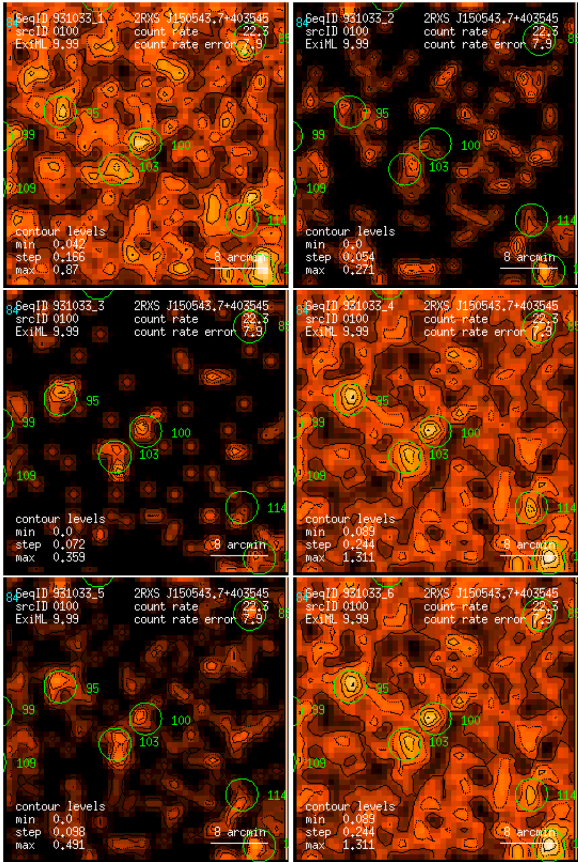
Figure 100: RASS 931033: detection 0100: band rate images, Gaussian filter: (1) PSPC channels 11 – 41, (2) 52 – 90, (3) 91 – 201, (4) 11 – 235, (5) 52 – 201, (6) 11 – 201. Broad band rates in counts/ks. Band rate contour levels in counts/ks/arcmin 2 .
