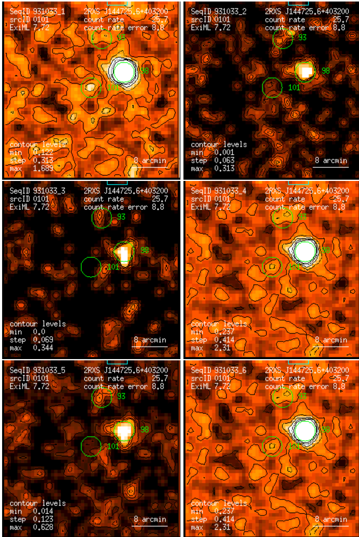
Figure 101: RASS 931033: detection 0101: band rate images, Gaussian filter: (1) PSPC channels 11 – 41, (2) 52 – 90, (3) 91 – 201, (4) 11 – 235, (5) 52 – 201, (6) 11 – 201. Broad band rates in counts/ks. Band rate contour levels in counts/ks/arcmin 2 .
