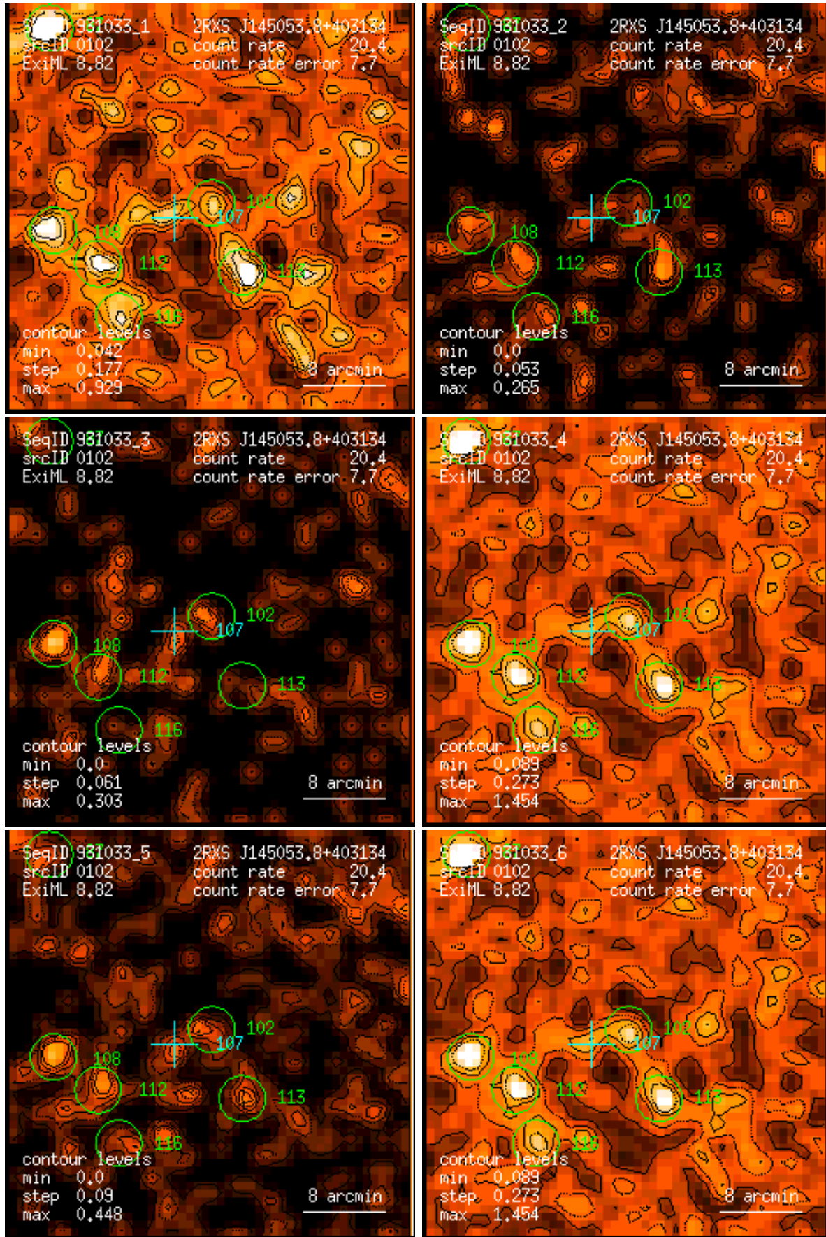
Figure 102: RASS 931033: detection 0102: band rate images, Gaussian filter: (1) PSPC channels 11 – 41, (2) 52 – 90, (3) 91 – 201, (4) 11 – 235, (5) 52 – 201, (6) 11 – 201. Broad band rates in counts/ks. Band rate contour levels in counts/ks/arcmin 2 .
