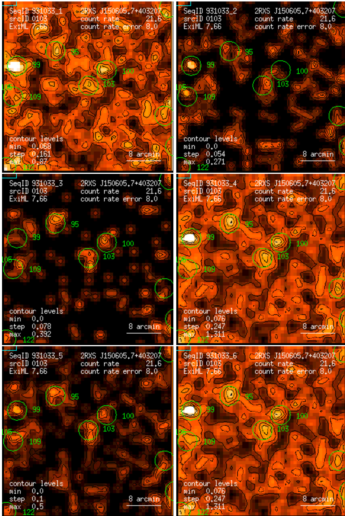
Figure 103: RASS 931033: detection 0103: band rate images, Gaussian filter: (1) PSPC channels 11 – 41, (2) 52 – 90, (3) 91 – 201, (4) 11 – 235, (5) 52 – 201, (6) 11 – 201. Broad band rates in counts/ks. Band rate contour levels in counts/ks/arcmin 2 .
