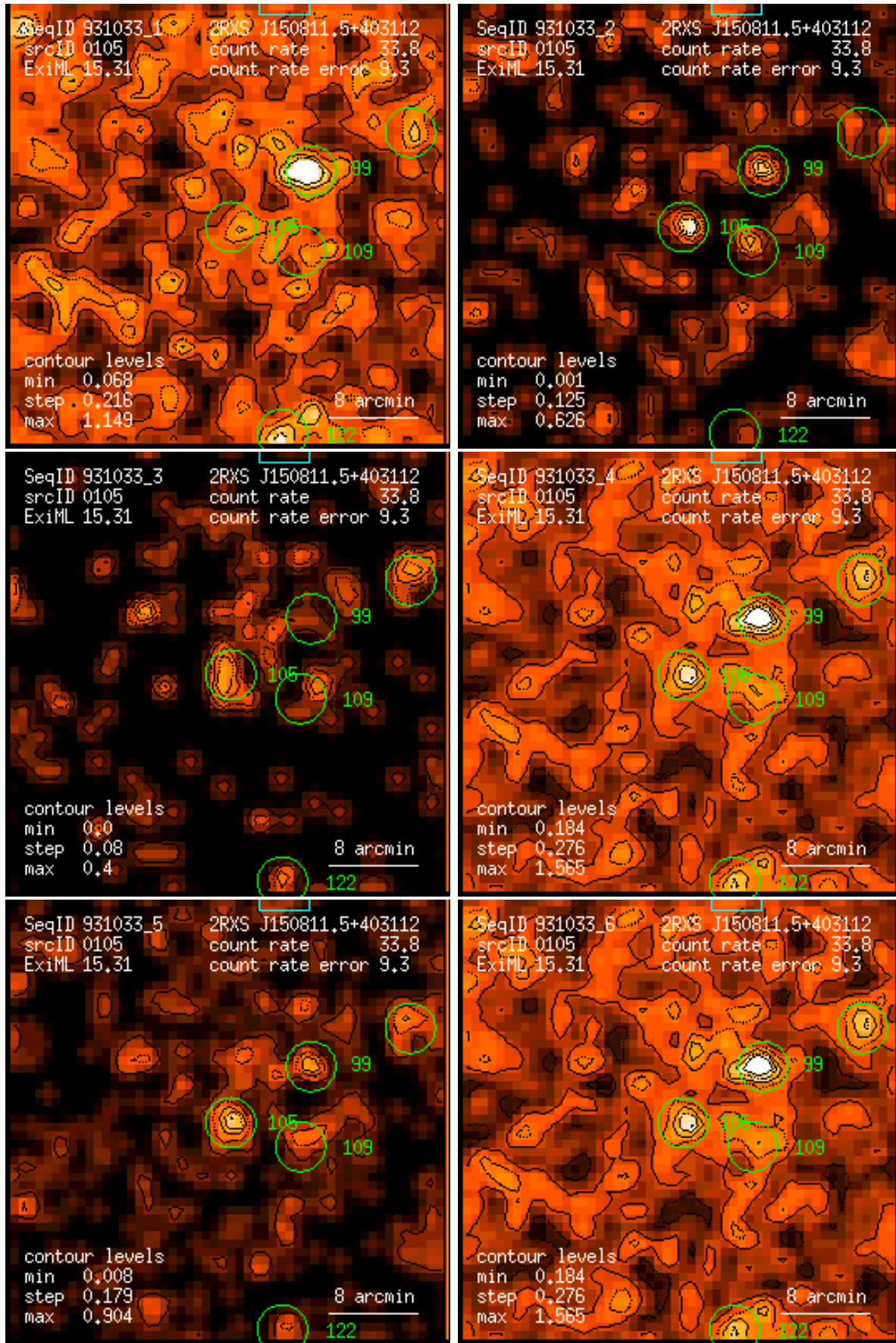
Figure 105: RASS 931033: detection 0105: band rate images, Gaussian filter: (1) PSPC channels 11 – 41, (2) 52 – 90, (3) 91 – 201, (4) 11 – 235, (5) 52 – 201, (6) 11 – 201. Broad band rates in counts/ks. Band rate contour levels in counts/ks/arcmin 2 .
