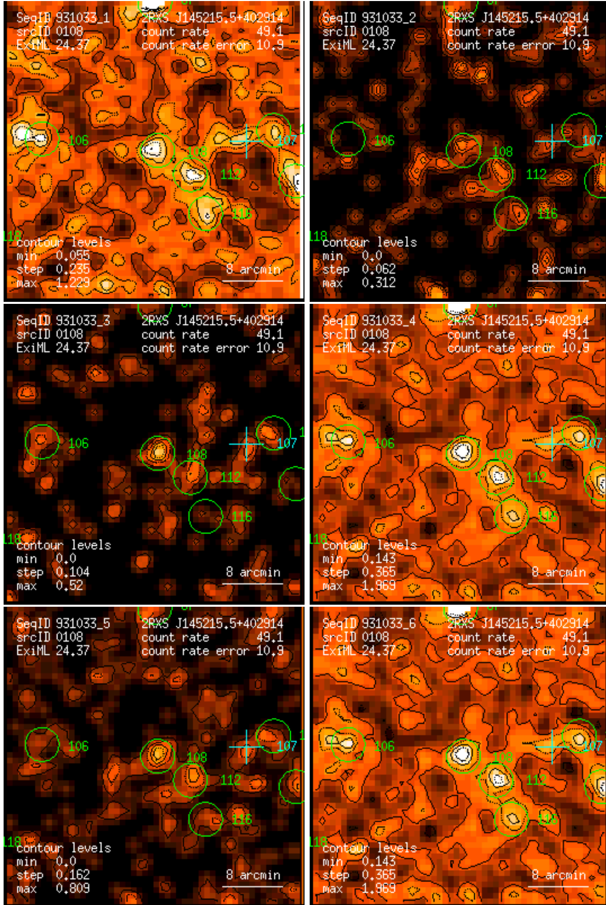
Figure 108: RASS 931033: detection 0108: band rate images, Gaussian filter: (1) PSPC channels 11 – 41, (2) 52 – 90, (3) 91 – 201, (4) 11 – 235, (5) 52 – 201, (6) 11 – 201. Broad band rates in counts/ks. Band rate contour levels in counts/ks/arcmin 2 .
