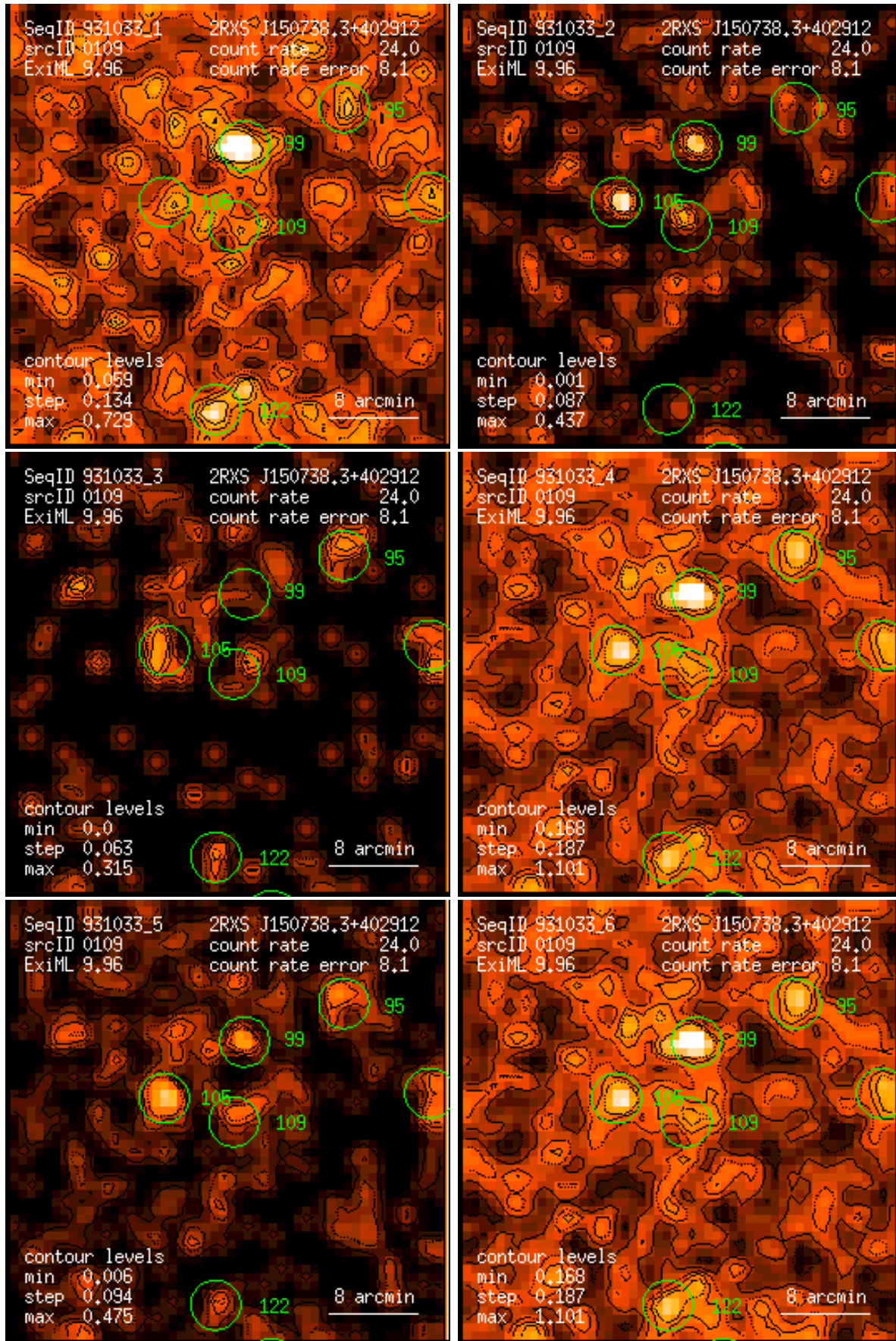
Figure 109: RASS 931033: detection 0109: band rate images, Gaussian filter: (1) PSPC channels 11 – 41, (2) 52 – 90, (3) 91 – 201, (4) 11 – 235, (5) 52 – 201, (6) 11 – 201. Broad band rates in counts/ks. Band rate contour levels in counts/ks/arcmin 2 .
