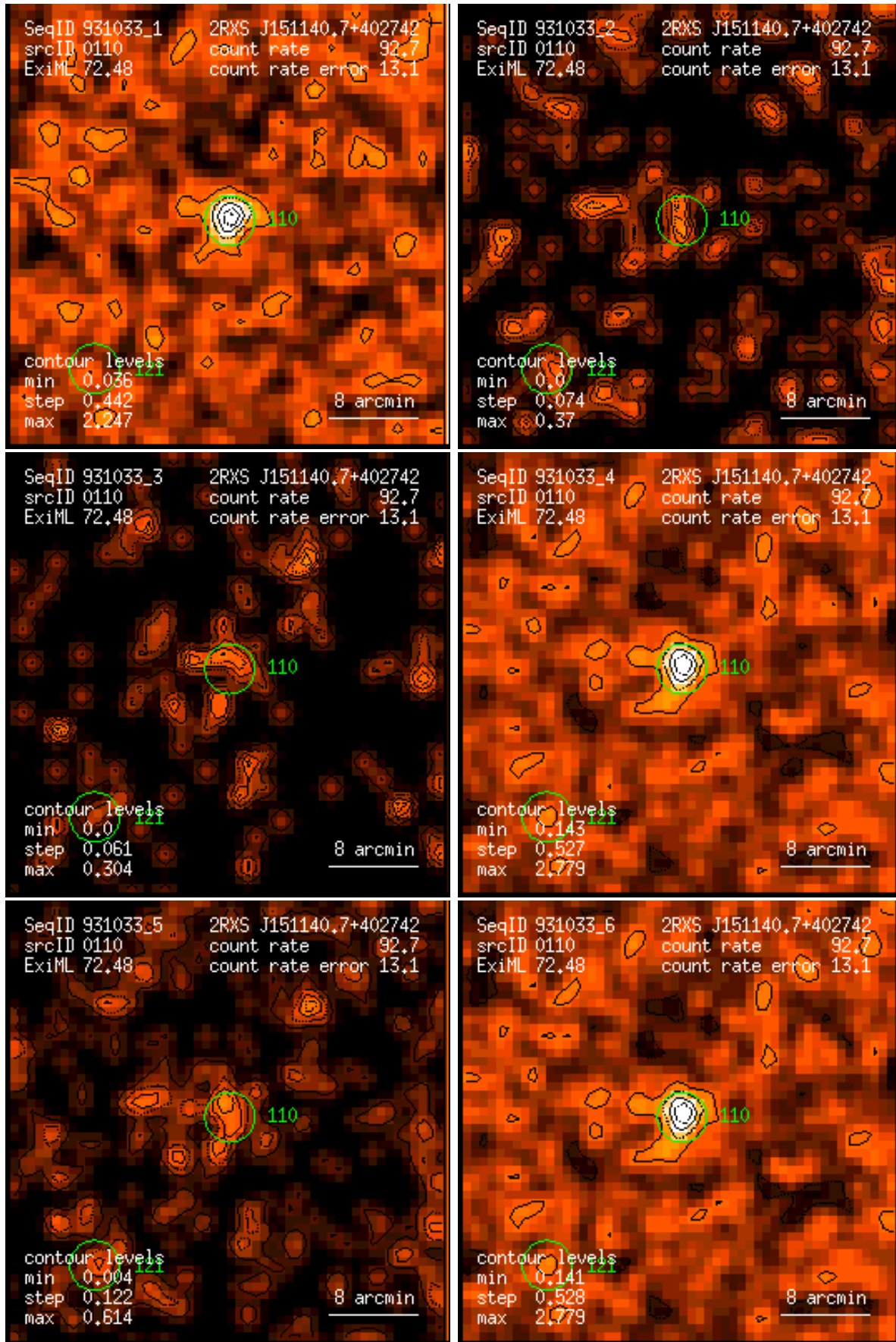
Figure 110: RASS 931033: detection 0110: band rate images, Gaussian filter: (1) PSPC channels 11 – 41, (2) 52 – 90, (3) 91 – 201, (4) 11 – 235, (5) 52 – 201, (6) 11 – 201. Broad band rates in counts/ks. Band rate contour levels in counts/ks/arcmin 2 .
