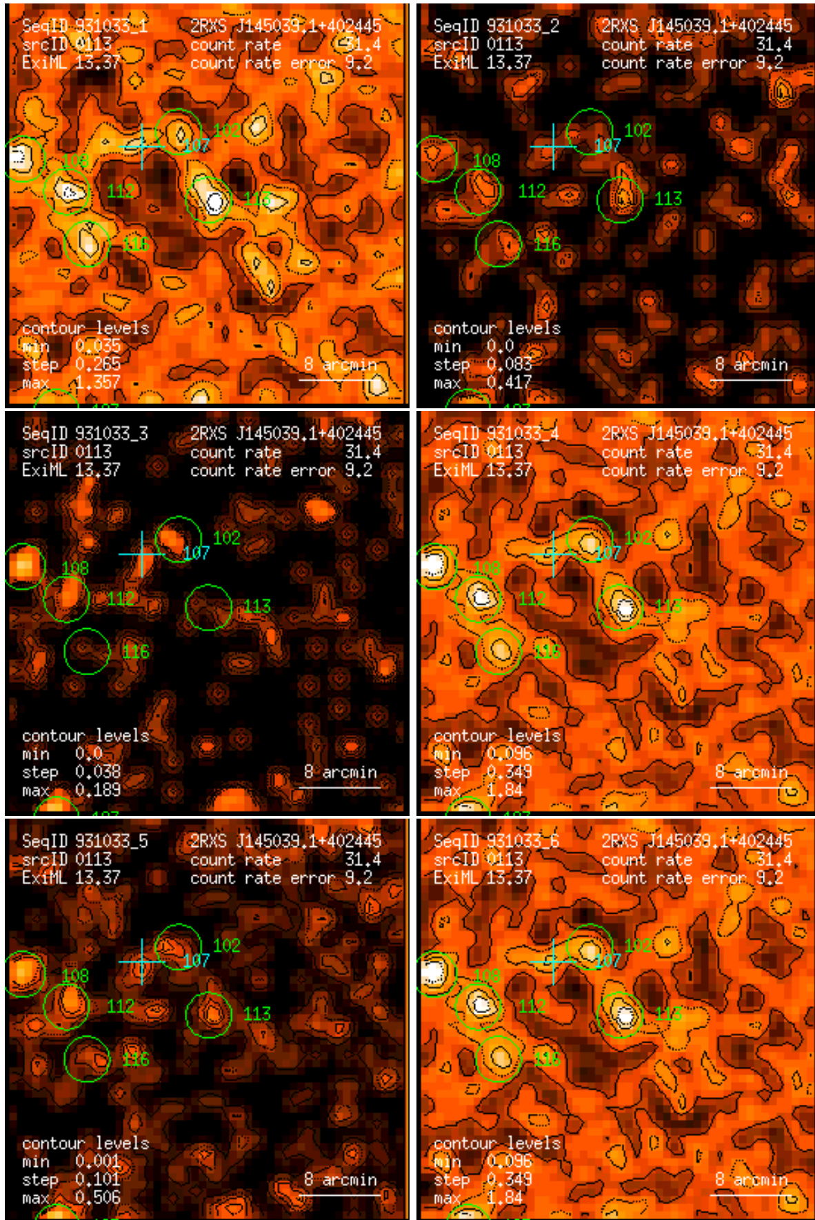
Figure 113: RASS 931033: detection 0113: band rate images, Gaussian filter: (1) PSPC channels 11 – 41, (2) 52 – 90, (3) 91 – 201, (4) 11 – 235, (5) 52 – 201, (6) 11 – 201. Broad band rates in counts/ks. Band rate contour levels in counts/ks/arcmin 2 .
