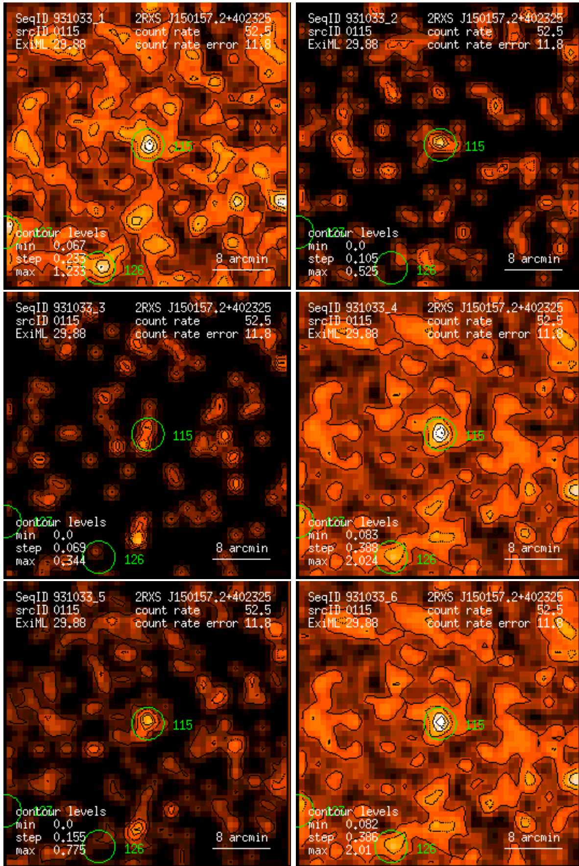
Figure 115: RASS 931033: detection 0115: band rate images, Gaussian filter: (1) PSPC channels 11 – 41, (2) 52 – 90, (3) 91 – 201, (4) 11 – 235, (5) 52 – 201, (6) 11 – 201. Broad band rates in counts/ks. Band rate contour levels in counts/ks/arcmin 2 .
