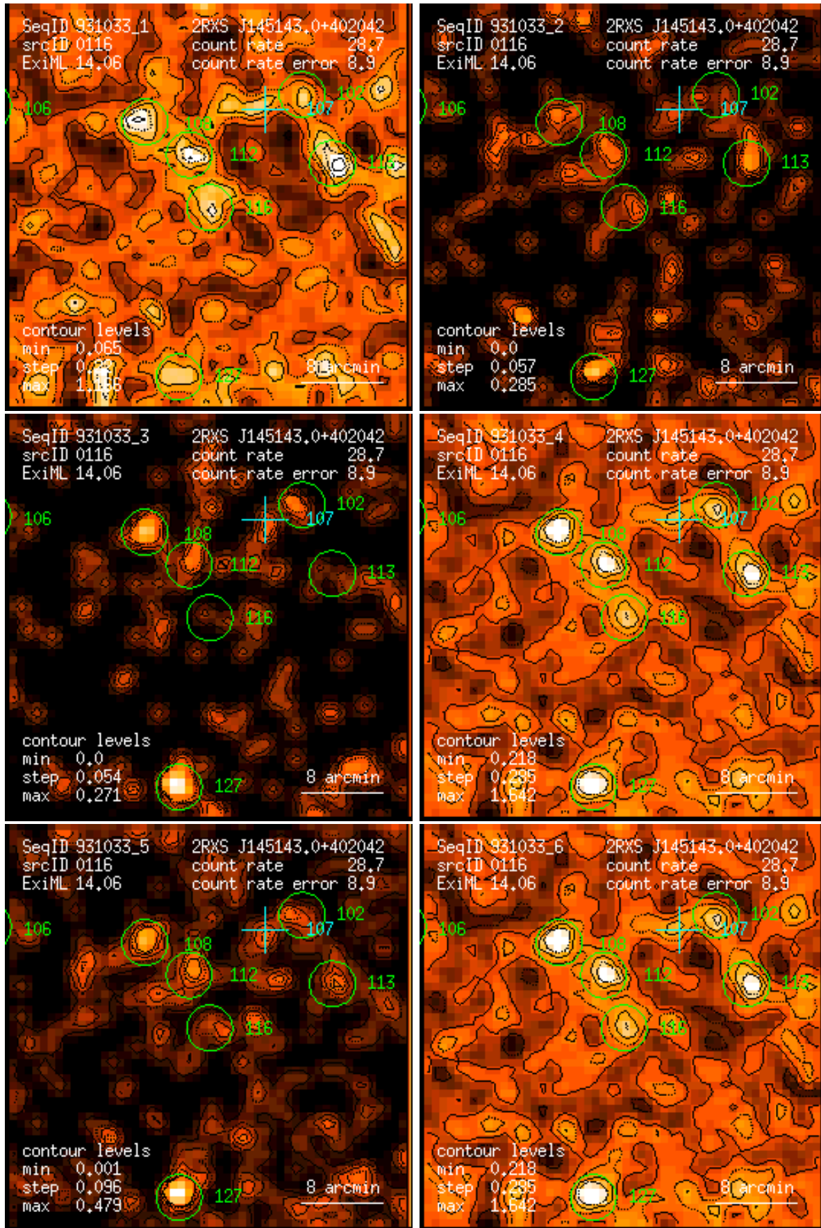
Figure 116: RASS 931033: detection 0116: band rate images, Gaussian filter: (1) PSPC channels 11 – 41, (2) 52 – 90, (3) 91 – 201, (4) 11 – 235, (5) 52 – 201, (6) 11 – 201. Broad band rates in counts/ks. Band rate contour levels in counts/ks/arcmin 2 .
