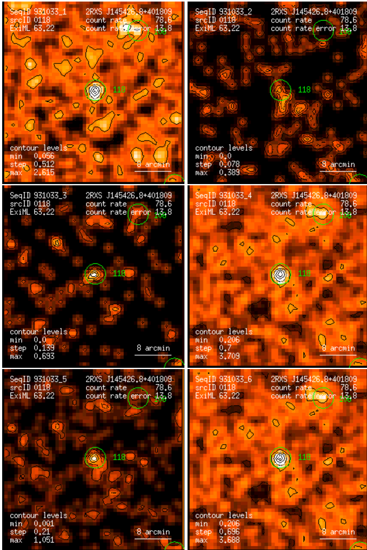
Figure 118: RASS 931033: detection 0118: band rate images, Gaussian filter: (1) PSPC channels 11 – 41, (2) 52 – 90, (3) 91 – 201, (4) 11 – 235, (5) 52 – 201, (6) 11 – 201. Broad band rates in counts/ks. Band rate contour levels in counts/ks/arcmin 2 .
