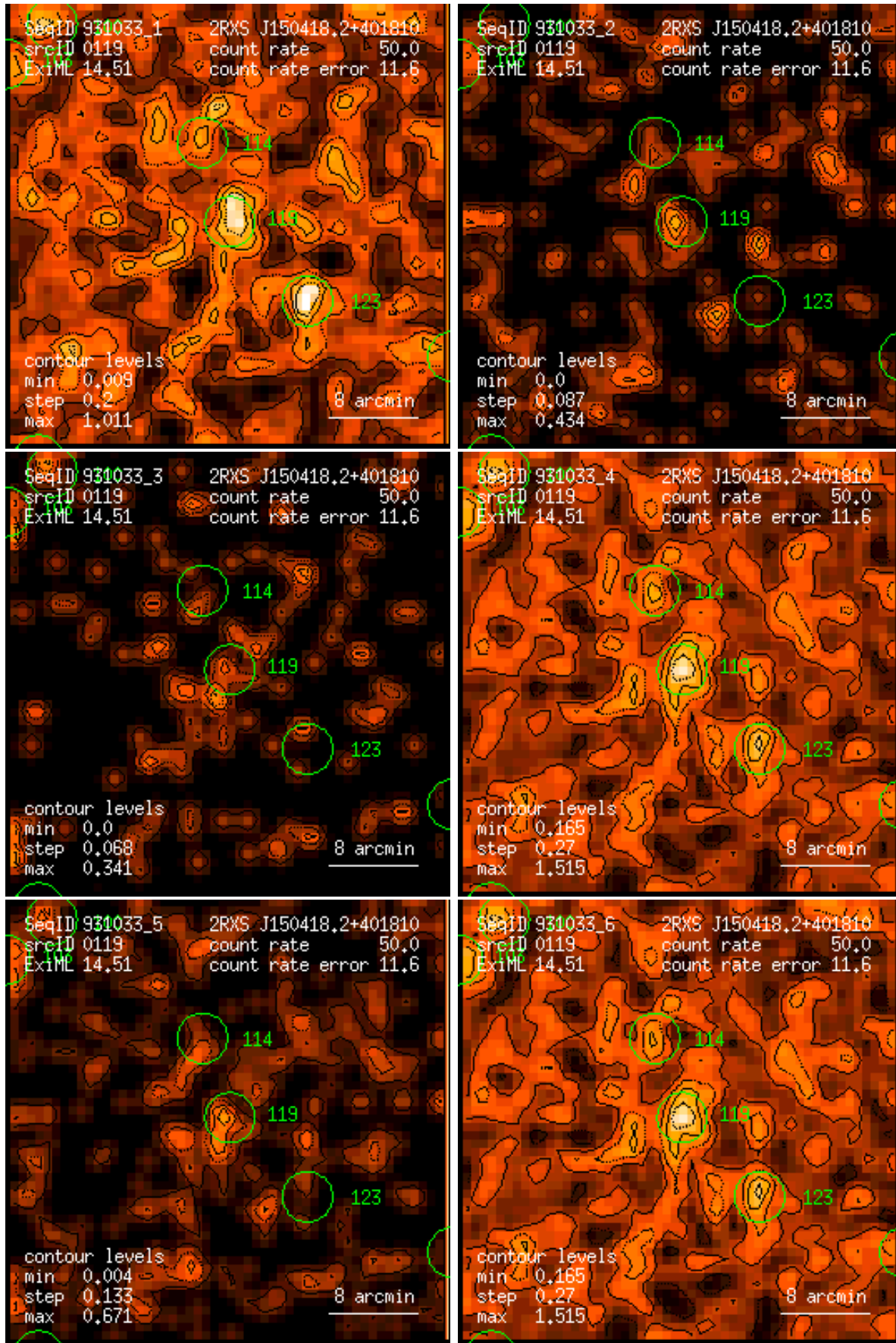
Figure 119: RASS 931033: detection 0119: band rate images, Gaussian filter: (1) PSPC channels 11 – 41, (2) 52 – 90, (3) 91 – 201, (4) 11 – 235, (5) 52 – 201, (6) 11 – 201. Broad band rates in counts/ks. Band rate contour levels in counts/ks/arcmin 2 .
