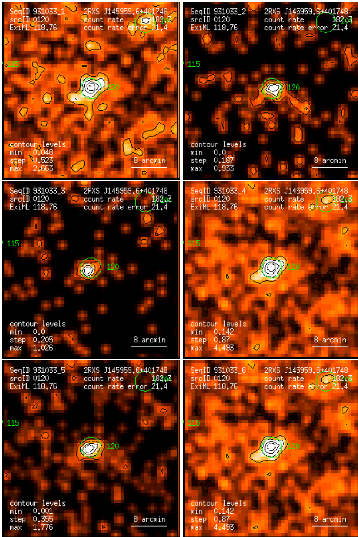
Figure 120: RASS 931033: detection 0120: band rate images, Gaussian filter: (1) PSPC channels 11 – 41, (2) 52 – 90, (3) 91 – 201, (4) 11 – 235, (5) 52 – 201, (6) 11 – 201. Broad band rates in counts/ks. Band rate contour levels in counts/ks/arcmin 2 .
