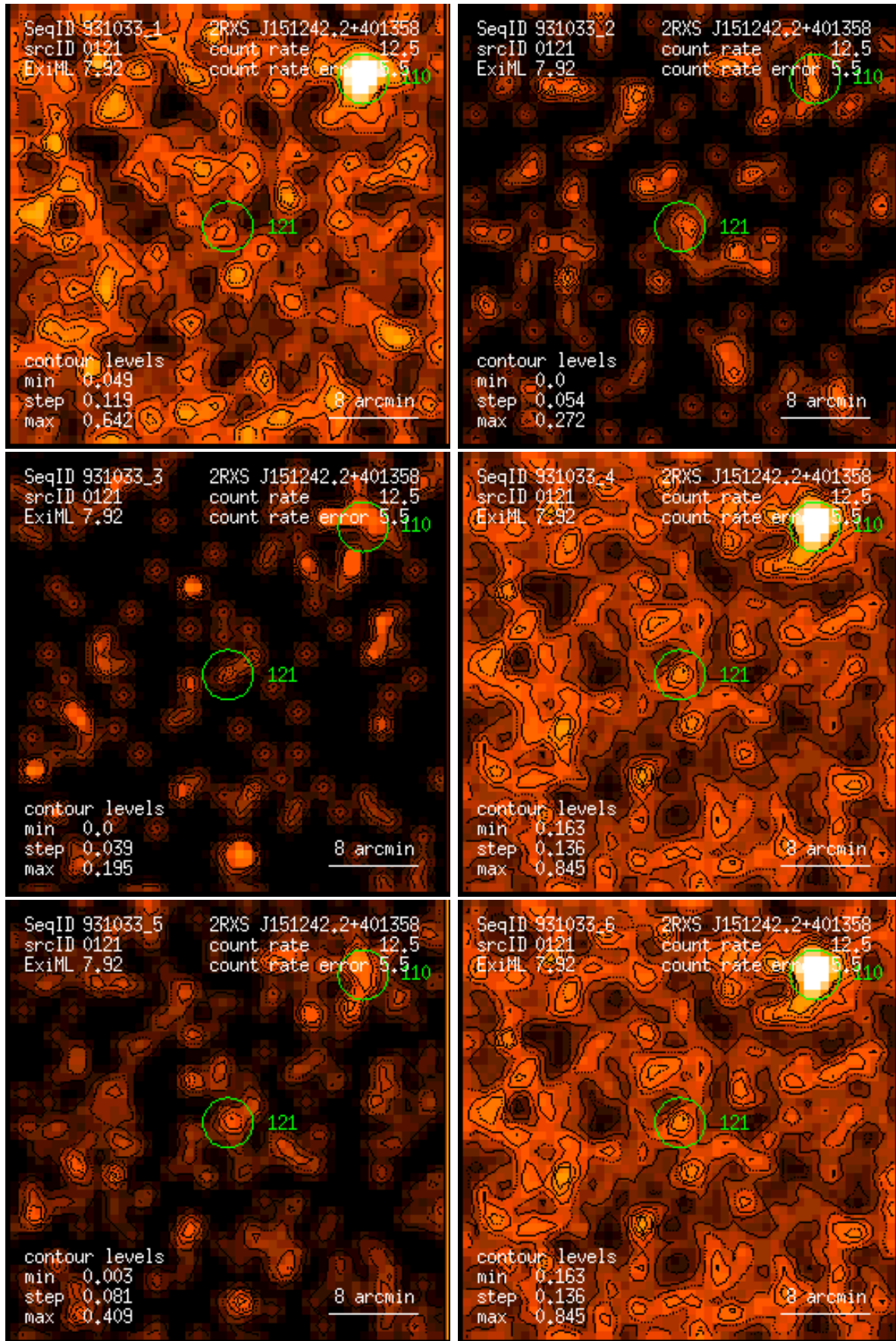
Figure 121: RASS 931033: detection 0121: band rate images, Gaussian filter: (1) PSPC channels 11 – 41, (2) 52 – 90, (3) 91 – 201, (4) 11 – 235, (5) 52 – 201, (6) 11 – 201. Broad band rates in counts/ks. Band rate contour levels in counts/ks/arcmin 2 .
