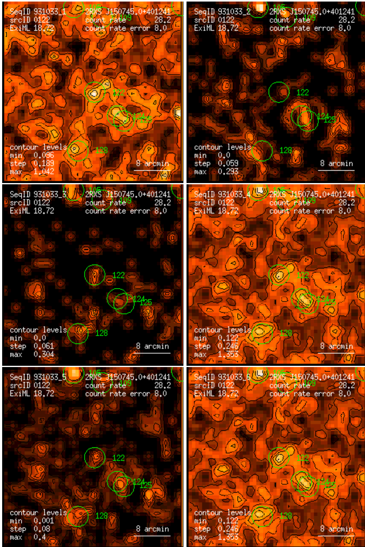
Figure 122: RASS 931033: detection 0122: band rate images, Gaussian filter: (1) PSPC channels 11 – 41, (2) 52 – 90, (3) 91 – 201, (4) 11 – 235, (5) 52 – 201, (6) 11 – 201. Broad band rates in counts/ks. Band rate contour levels in counts/ks/arcmin 2 .
