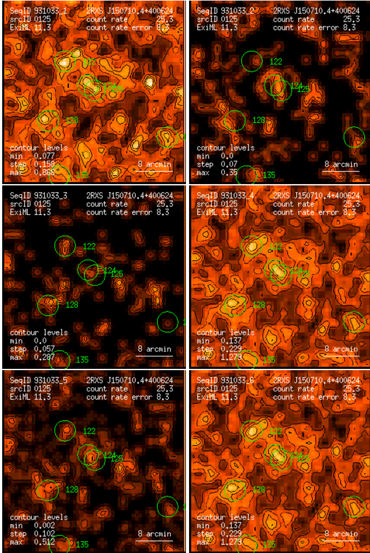
Figure 125: RASS 931033: detection 0125: band rate images, Gaussian filter: (1) PSPC channels 11 – 41, (2) 52 – 90, (3) 91 – 201, (4) 11 – 235, (5) 52 – 201, (6) 11 – 201. Broad band rates in counts/ks. Band rate contour levels in counts/ks/arcmin 2 .
