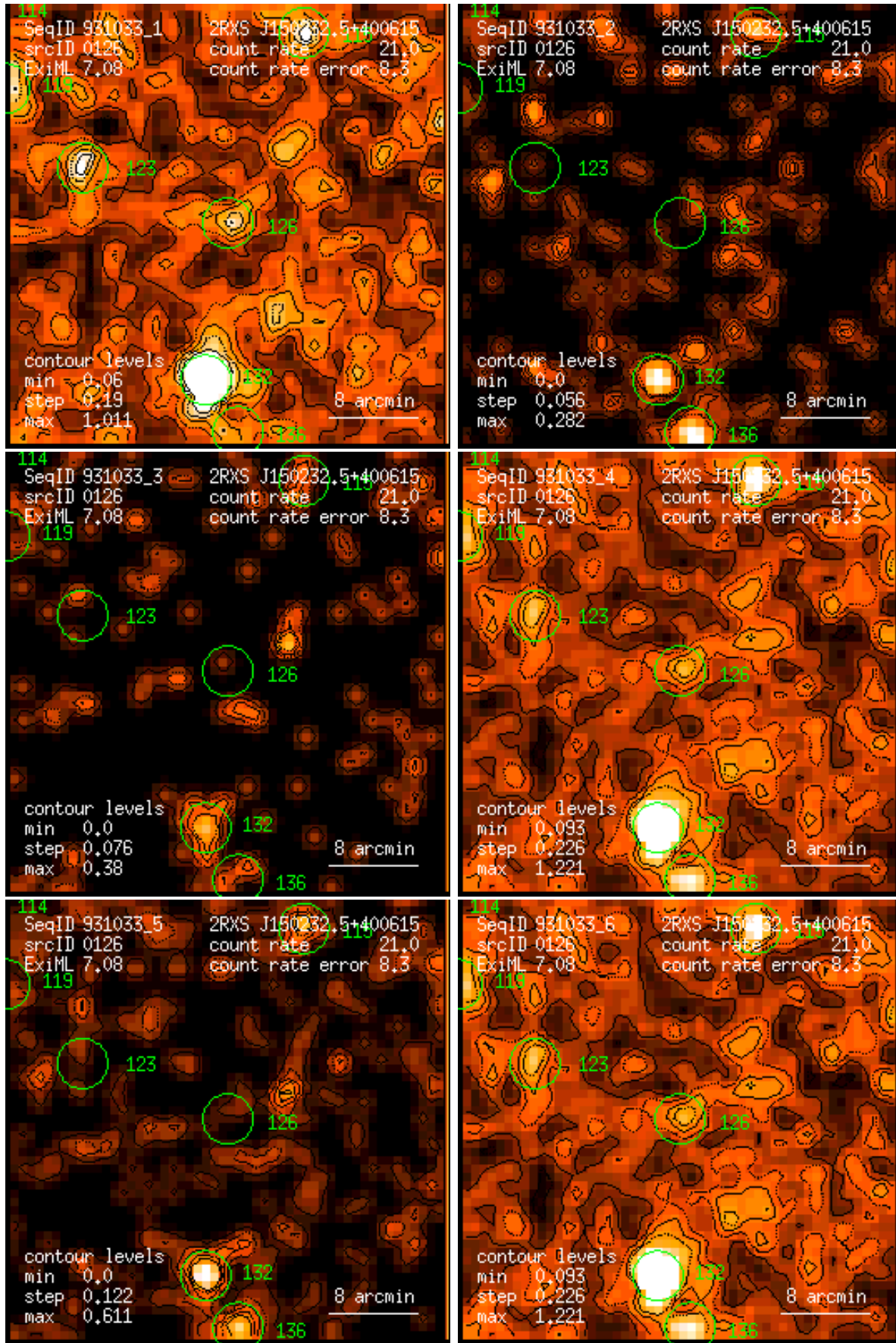
Figure 126: RASS 931033: detection 0126: band rate images, Gaussian filter: (1) PSPC channels 11 – 41, (2) 52 – 90, (3) 91 – 201, (4) 11 – 235, (5) 52 – 201, (6) 11 – 201. Broad band rates in counts/ks. Band rate contour levels in counts/ks/arcmin 2 .
