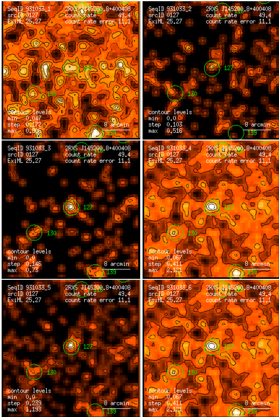
Figure 127: RASS 931033: detection 0127: band rate images, Gaussian filter: (1) PSPC channels 11 – 41, (2) 52 – 90, (3) 91 – 201, (4) 11 – 235, (5) 52 – 201, (6) 11 – 201. Broad band rates in counts/ks. Band rate contour levels in counts/ks/arcmin 2 .
