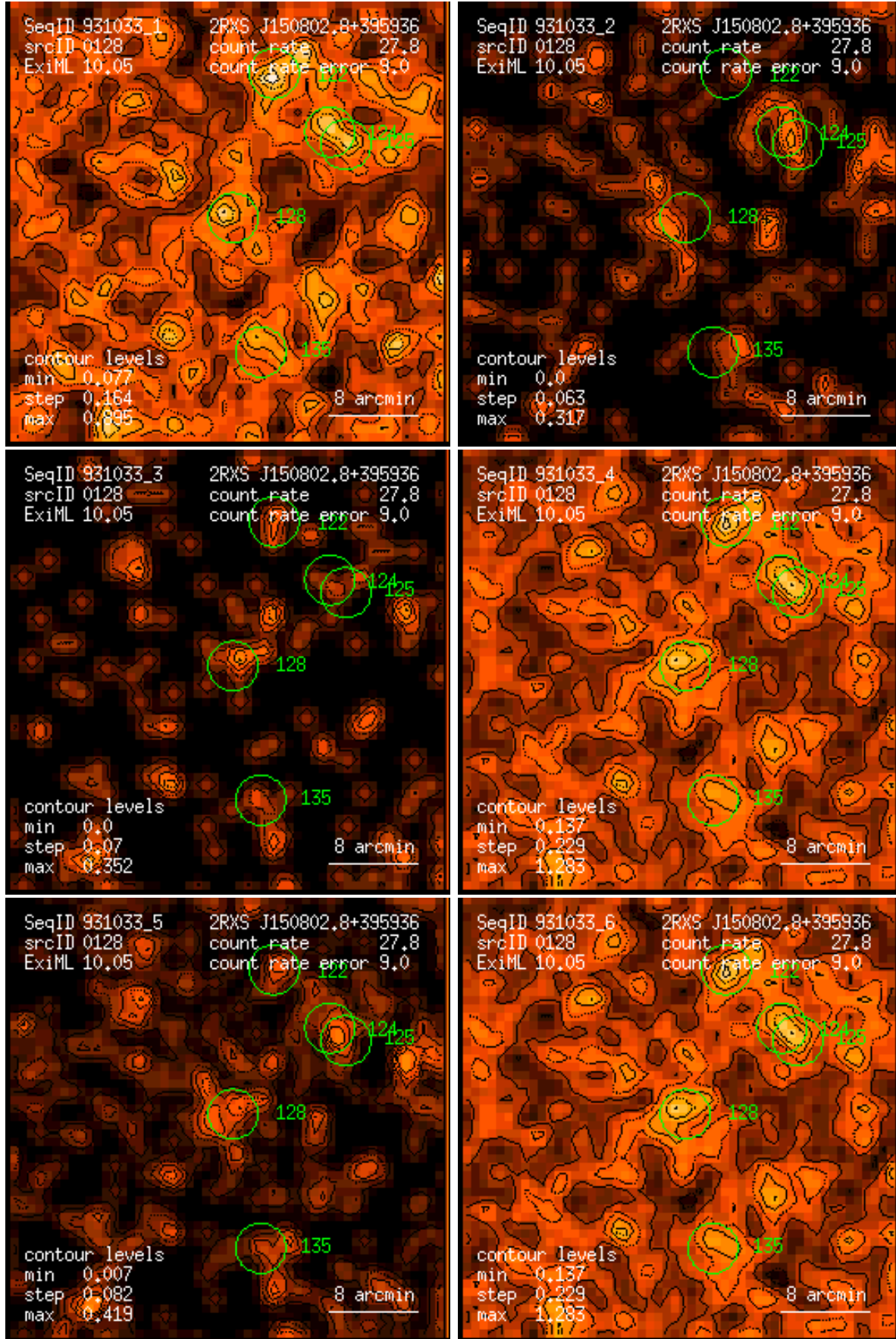
Figure 128: RASS 931033: detection 0128: band rate images, Gaussian filter: (1) PSPC channels 11 – 41, (2) 52 – 90, (3) 91 – 201, (4) 11 – 235, (5) 52 – 201, (6) 11 – 201. Broad band rates in counts/ks. Band rate contour levels in counts/ks/arcmin 2 .
