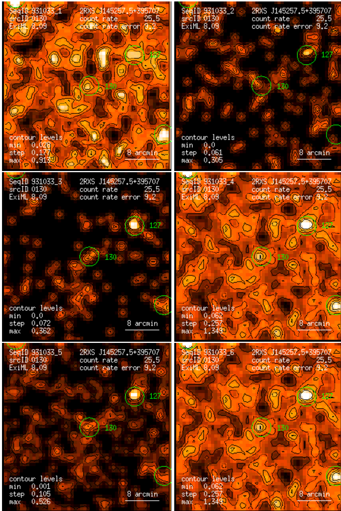
Figure 130: RASS 931033: detection 0130: band rate images, Gaussian filter: (1) PSPC channels 11 – 41, (2) 52 – 90, (3) 91 – 201, (4) 11 – 235, (5) 52 – 201, (6) 11 – 201. Broad band rates in counts/ks. Band rate contour levels in counts/ks/arcmin 2 .
