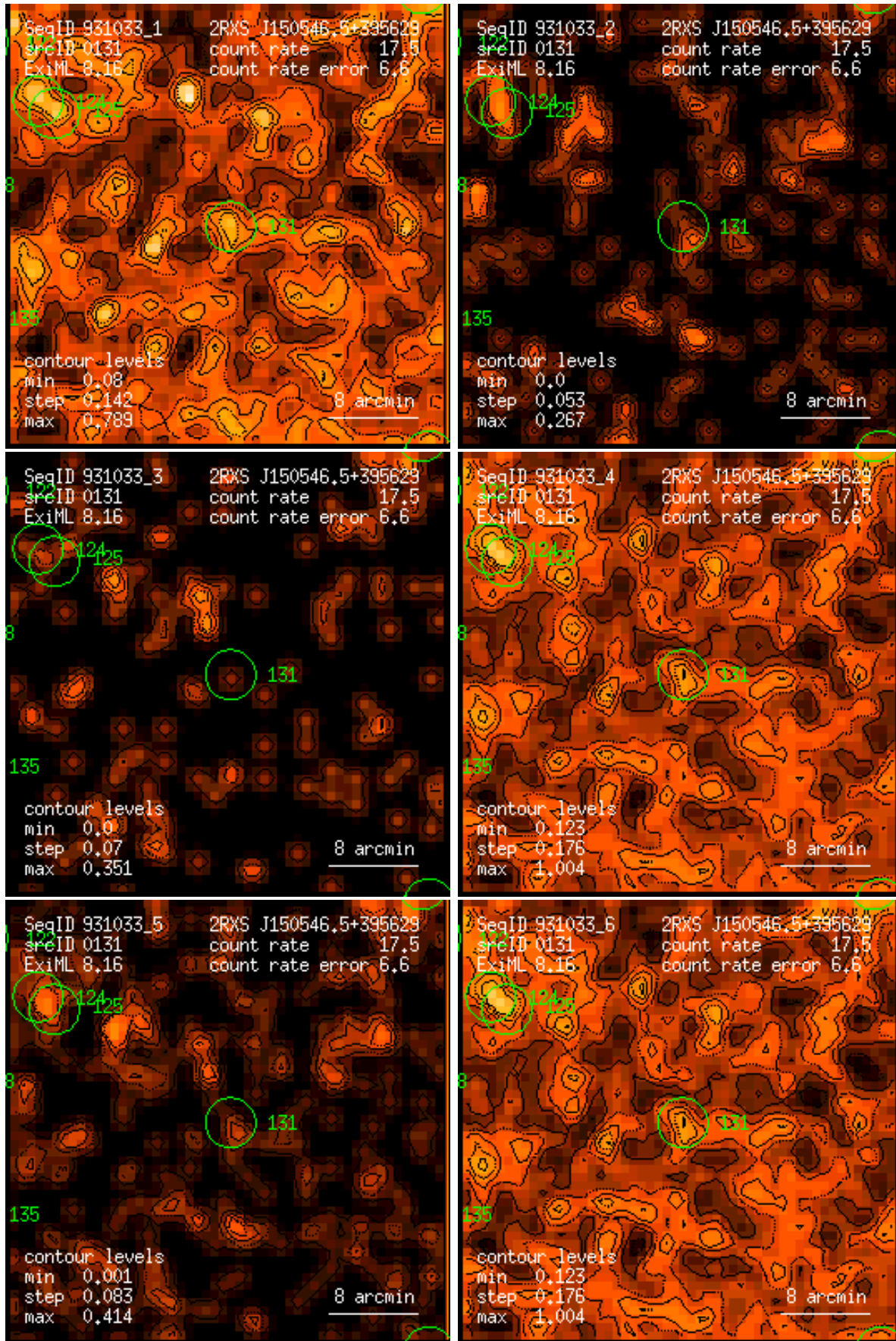
Figure 131: RASS 931033: detection 0131: band rate images, Gaussian filter: (1) PSPC channels 11 – 41, (2) 52 – 90, (3) 91 – 201, (4) 11 – 235, (5) 52 – 201, (6) 11 – 201. Broad band rates in counts/ks. Band rate contour levels in counts/ks/arcmin 2 .
