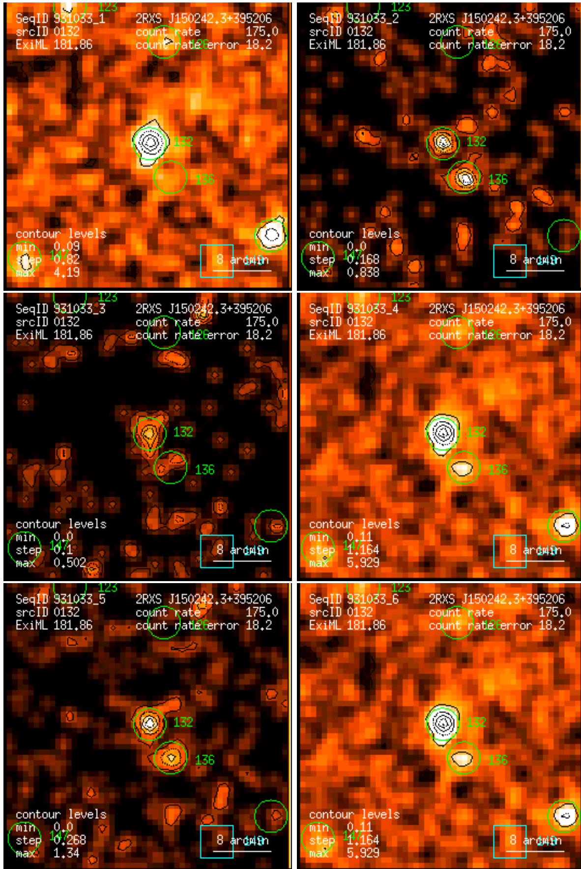
Figure 132: RASS 931033: detection 0132: band rate images, Gaussian filter: (1) PSPC channels 11 – 41, (2) 52 – 90, (3) 91 – 201, (4) 11 – 235, (5) 52 – 201, (6) 11 – 201. Broad band rates in counts/ks. Band rate contour levels in counts/ks/arcmin 2 .
