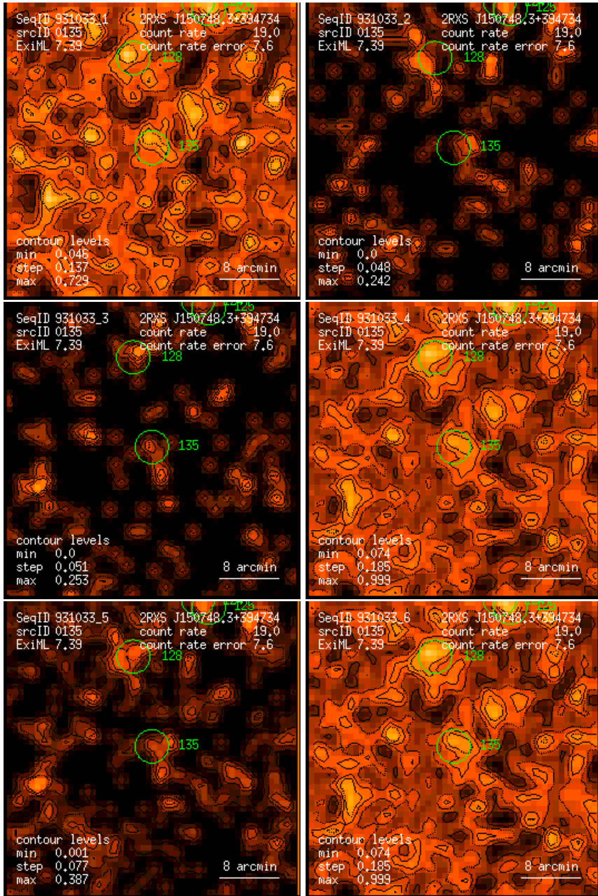
Figure 135: RASS 931033: detection 0135: band rate images, Gaussian filter: (1) PSPC channels 11 – 41, (2) 52 – 90, (3) 91 – 201, (4) 11 – 235, (5) 52 – 201, (6) 11 – 201. Broad band rates in counts/ks. Band rate contour levels in counts/ks/arcmin 2 .
