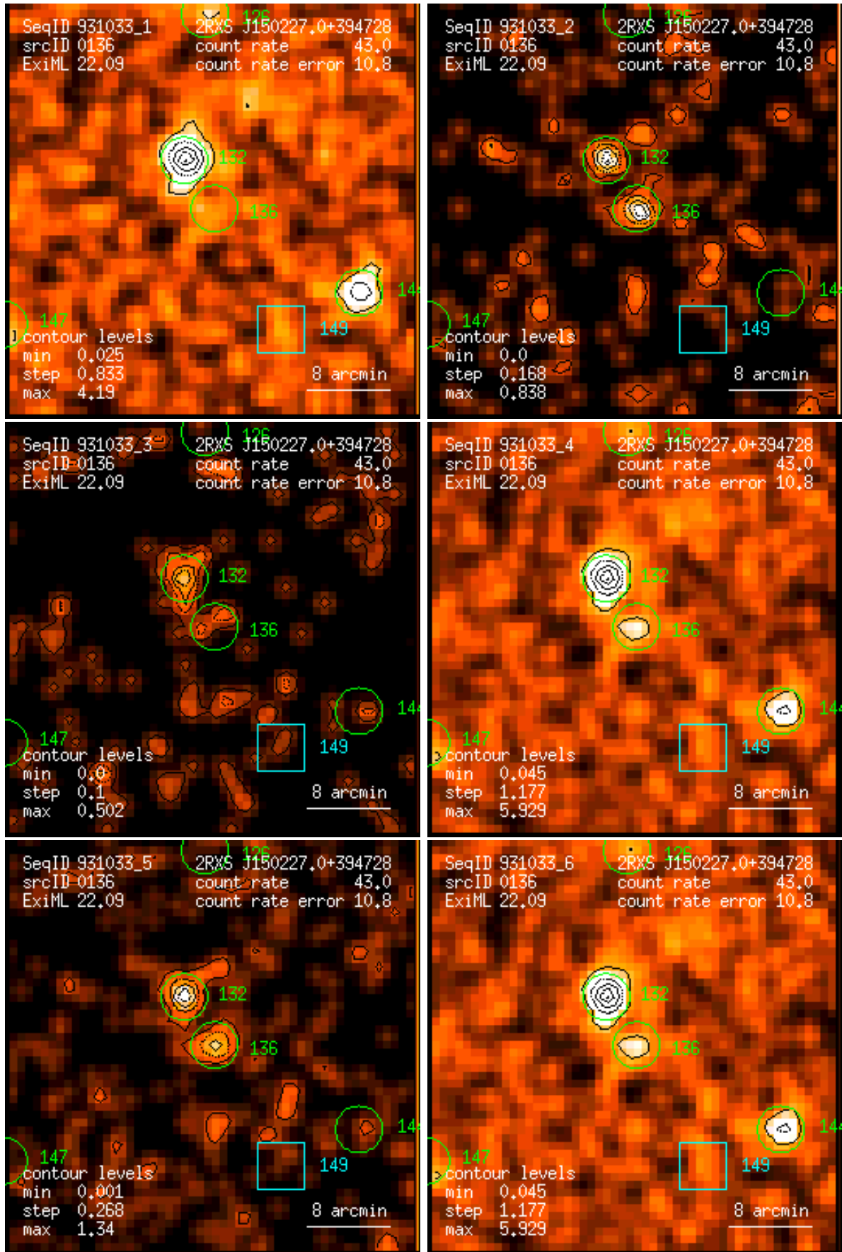
Figure 136: RASS 931033: detection 0136: band rate images, Gaussian filter: (1) PSPC channels 11 – 41, (2) 52 – 90, (3) 91 – 201, (4) 11 – 235, (5) 52 – 201, (6) 11 – 201. Broad band rates in counts/ks. Band rate contour levels in counts/ks/arcmin 2 .
