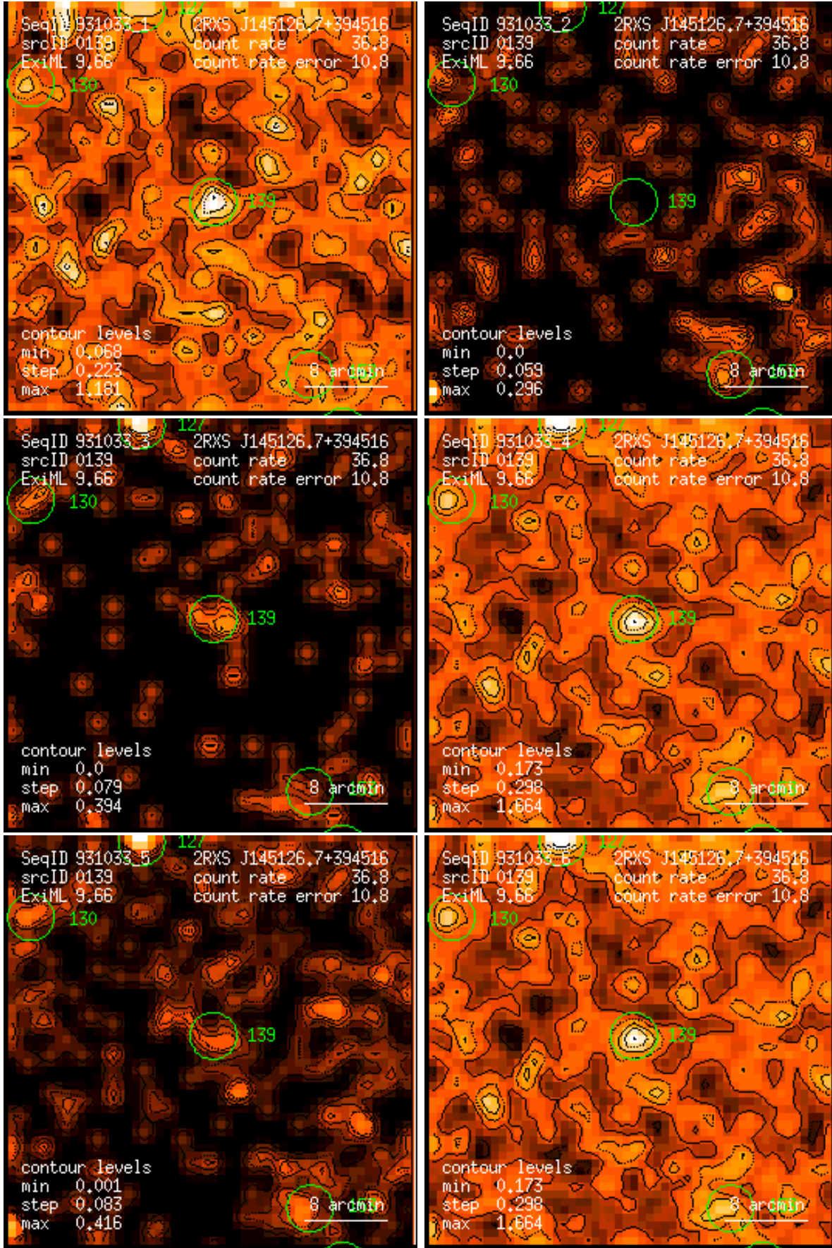
Figure 139: RASS 931033: detection 0139: band rate images, Gaussian filter: (1) PSPC channels 11 – 41, (2) 52 – 90, (3) 91 – 201, (4) 11 – 235, (5) 52 – 201, (6) 11 – 201. Broad band rates in counts/ks. Band rate contour levels in counts/ks/arcmin 2 .
