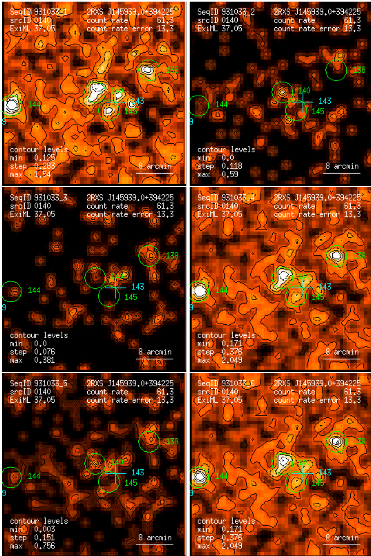
Figure 140: RASS 931033: detection 0140: band rate images, Gaussian filter: (1) PSPC channels 11 – 41, (2) 52 – 90, (3) 91 – 201, (4) 11 – 235, (5) 52 – 201, (6) 11 – 201. Broad band rates in counts/ks. Band rate contour levels in counts/ks/arcmin 2 .
