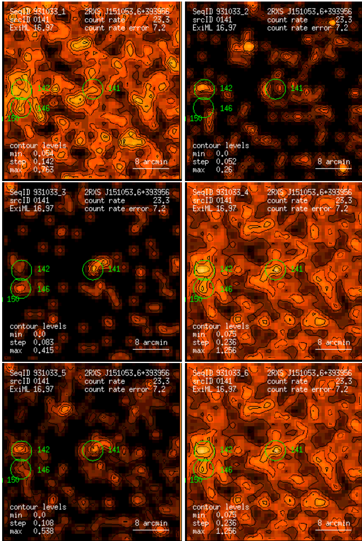
Figure 141: RASS 931033: detection 0141: band rate images, Gaussian filter: (1) PSPC channels 11 – 41, (2) 52 – 90, (3) 91 – 201, (4) 11 – 235, (5) 52 – 201, (6) 11 – 201. Broad band rates in counts/ks. Band rate contour levels in counts/ks/arcmin 2 .
